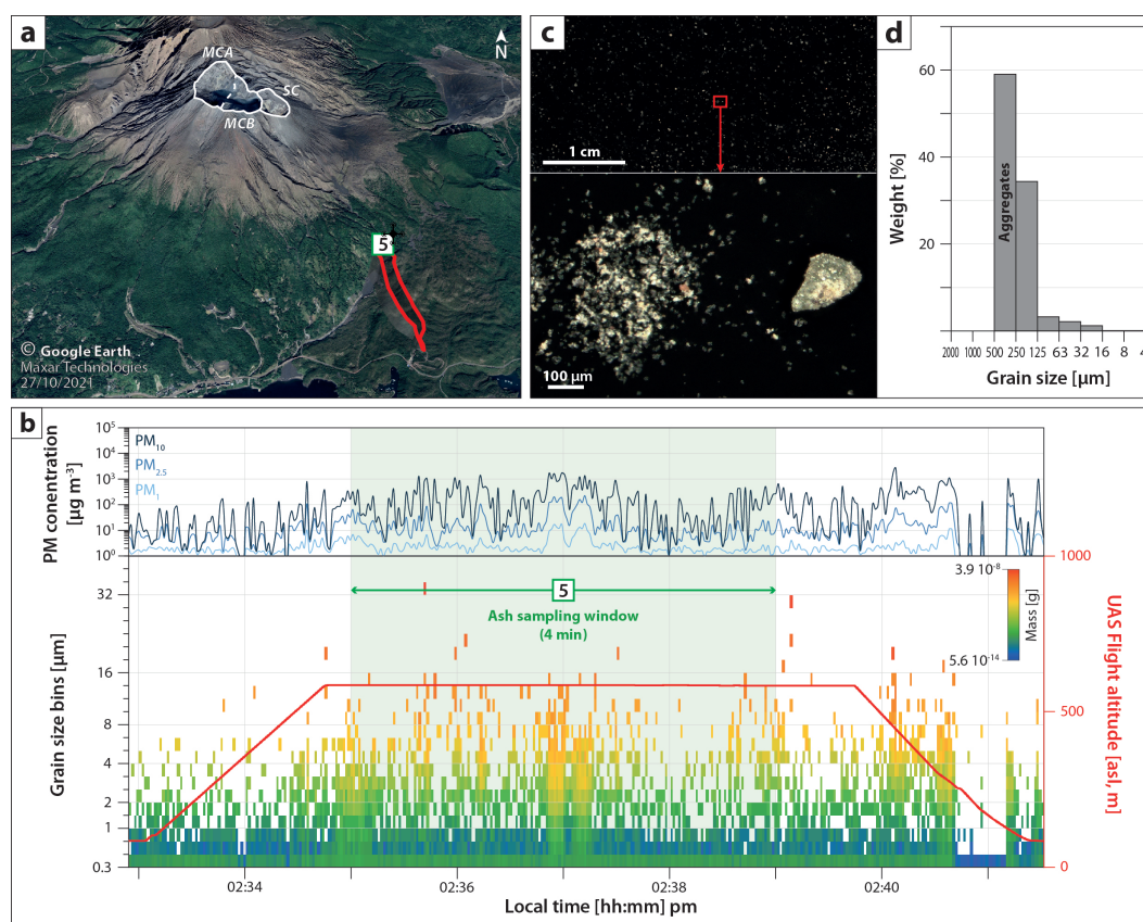
Figure 7. Results obtained by the \text{A}_2\text{C}_2 device for the 11 th of November 2023 explosive event at Sakurajima. (a) UAV flight path (red line) during which the optical particle counter (OPC) analysis was performed. The green square labeled 5 corresponds to the site shown in Figures 3c and 5b, and represents the ash sampling location and duration (also shown in b). White lines delimit the active craters shown in Figure 3b (MCA: Minamidake crater vent A; MCB: Minamidake crater vent B; SC: Showa crater). (b) Particulate matter (PM) concentrations and grain size spectrogram from the optical particle counter (OPC) data. (c) Optical microscopy images of the collected sample at different scales. (d) Grain Size Distribution (GSD) inferred from image analysis of the collected sample.
