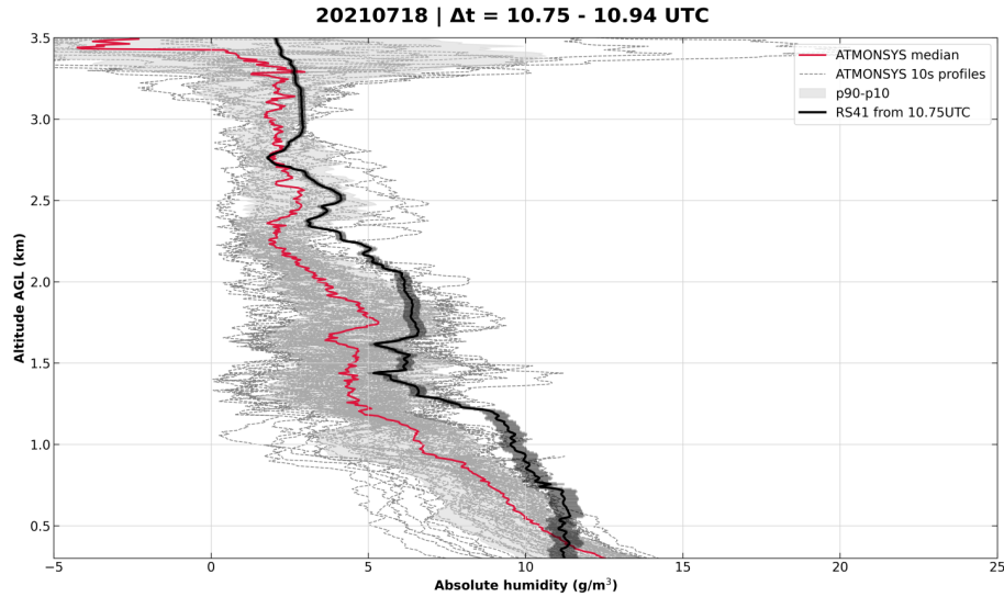
Figure 12. Inter-comparison between a radiosonde ascent and the ATMONSYS DIAL during the time of ascent from ground level to \approx 3.5 km above ground level. Statistical uncertainties for the radiosonde are represented by black shading.
