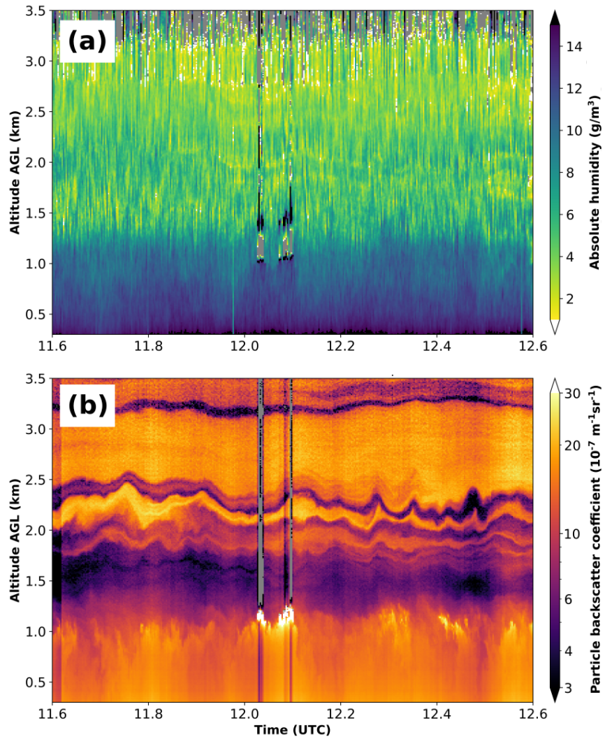
Figure 6. ATMONSYS lidar data showcase from 18 July 2021 for vertical and temporal highly resolved time series of (a) absolute humidity and (b) aerosol backscatter coefficients during high noon under clear-sky conditions and a temporal resolution of \Delta t = 10\text{s} . No temporal smoothing has been applied.
