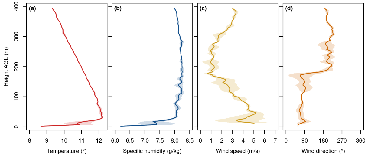
Figure 10. Exemplary synthesis plot showing air temperature (a), specific humidity (b), wind speed (c), and wind direction (d) profiles from the 16:55 sounding on 16 June 2021. Shaded areas indicate the standard deviation between the two consecutive descents of this sounding.
