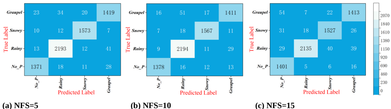
Figure 9: Confusion matrix of proposed algorithm. No_P means No precipitation. The three subplots share the same legend on the far right.
