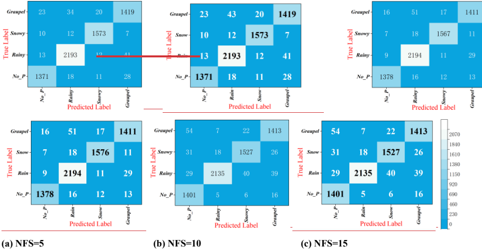
Figure 9: Confusion matrix of proposed algorithm. No_P means No precipitation. The three subplots share the same legend on the far right.
