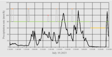
(c) Night-time Rain of camera_2
