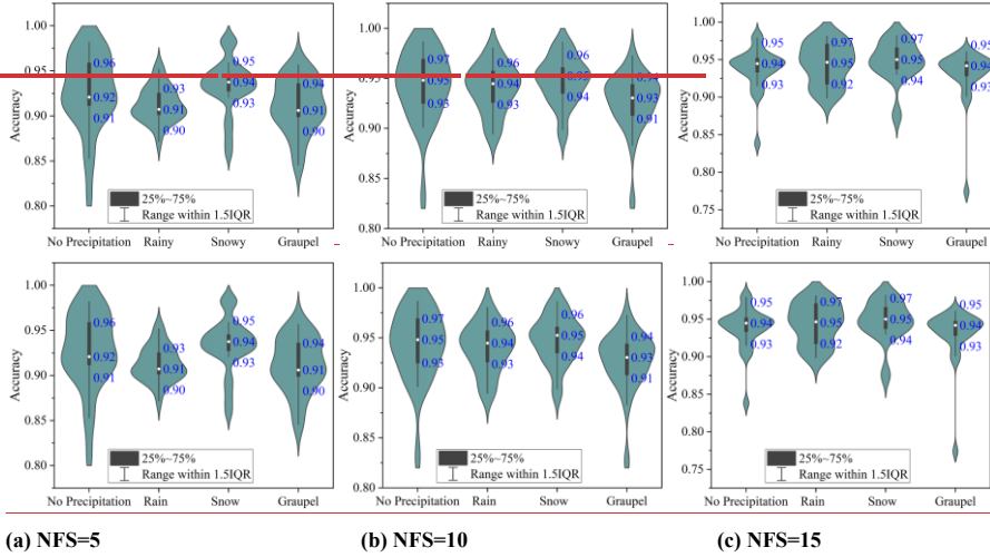
Figure 10: Violin plots quantify the deep-learning algorithms' performance for SPT classification.
