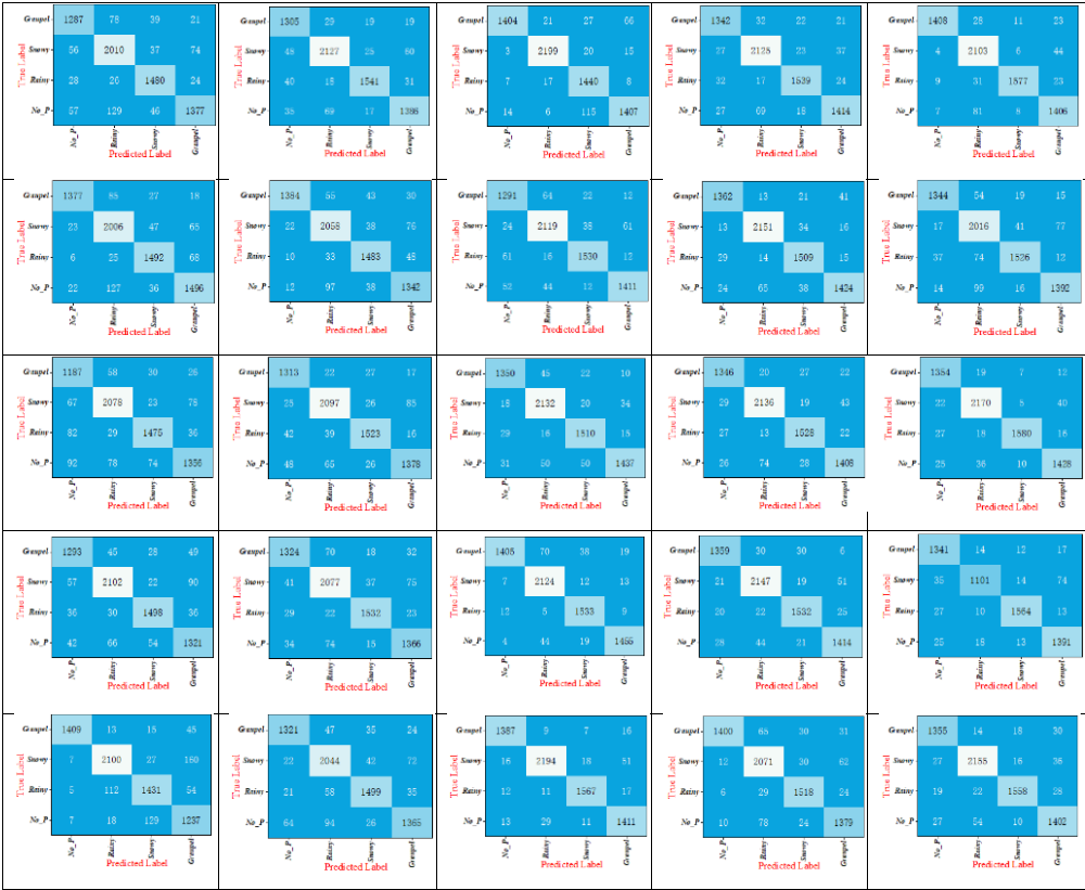
Note: First row: DenseNet 121; Second row: EfficientNet B0; Third row: Inception V3; Forth row: ResNet 50; Fifth Row: MobileNet V2.
