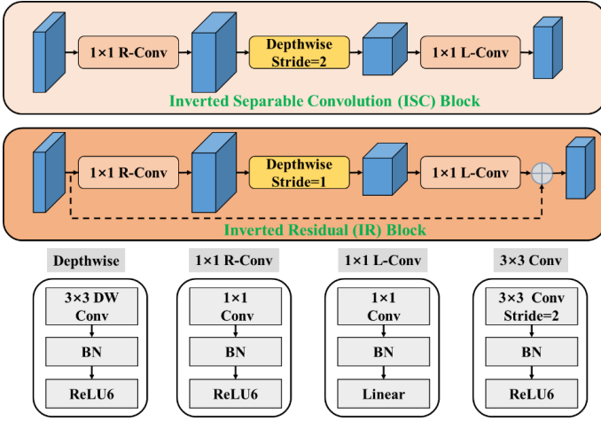
300 Figure 5: The structure of the inverted separable convolution (ISC) block and inverted residual (IR) block.
