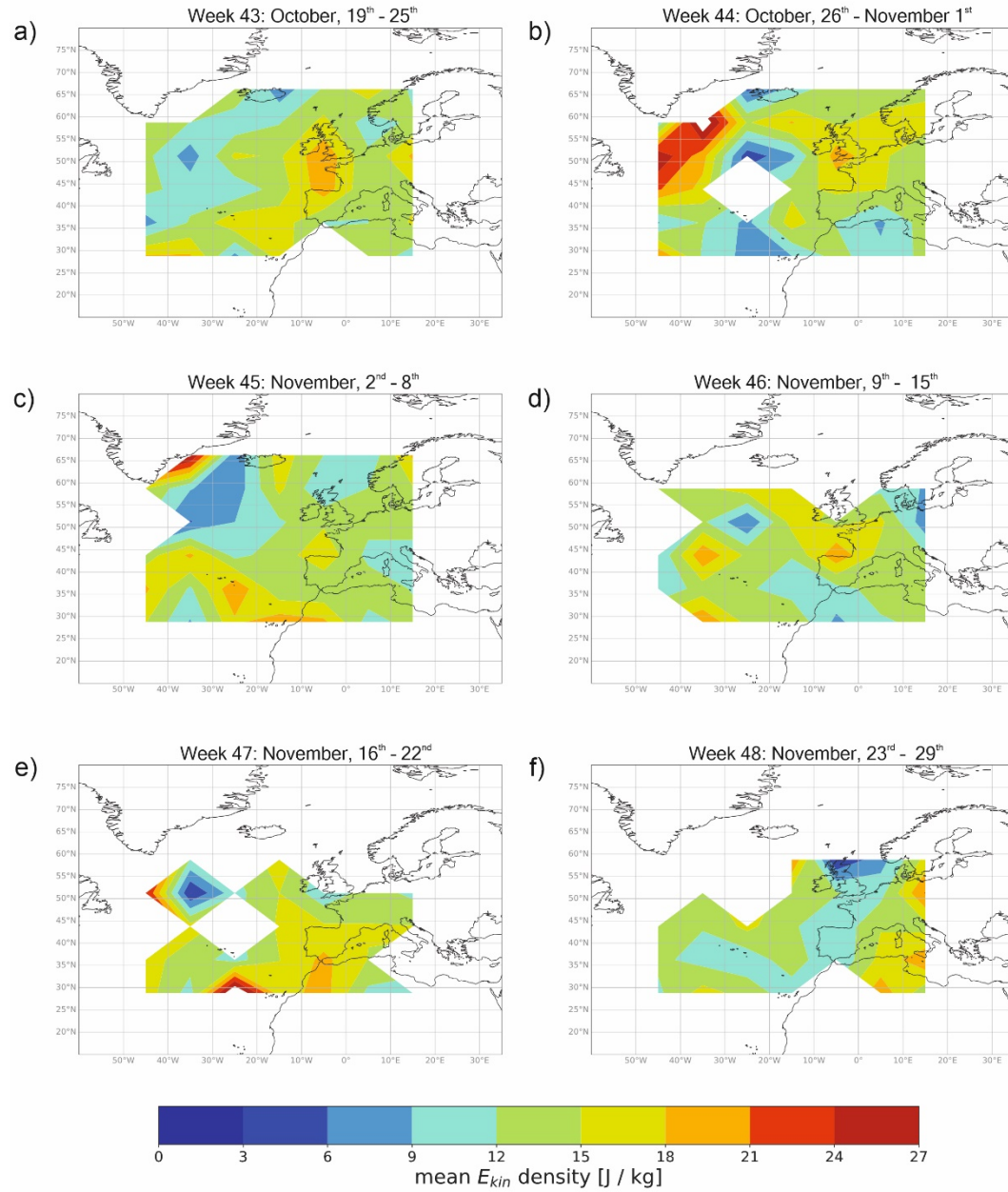
Figure 10 Development of the spatially resolved lower bound of the kinetic energy density averaged for the height range above 11 km with calendar week (CW), a) CW 43: October, 19 th – 25 th , b) CW 44: Oct. 26 th – Nov. 1 st , c) CW 45: Nov., 2 nd – 8 th , d) CW 46: Nov., 9 th – 15 th , e) CW 47: Nov., 16 th – 22 nd , f) CW 48: Nov., 23 rd – 29 th . The spatial resolution is 10° in zonal direction and 7.5° in meridional direction.
