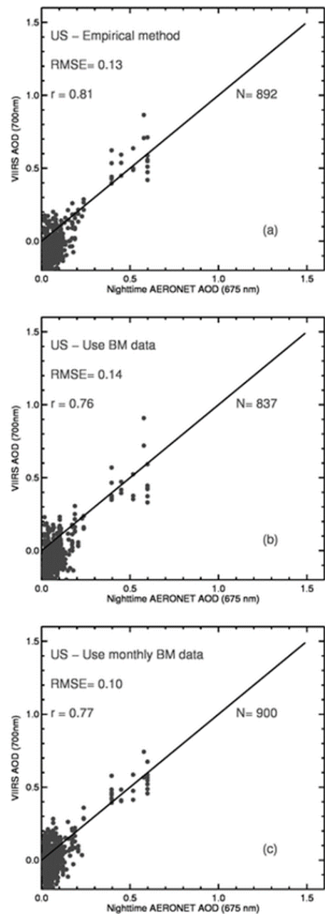
390 Figure 4. a) Scatter plot of nighttime AOTs derived from VIIRS/DNB (700 nm) and AERONET (675 nm) over the USA region. \Delta I_a values were estimated using the empirically-based method. Also shown is the one-to-one line. b) Similar to a) but using the yearly averaged monthly NASA’s VNP46 data to estimate \Delta I_a values. c) Similar to b) but using the monthly NASA’s VNP46 data to estimate \Delta I_a values.
