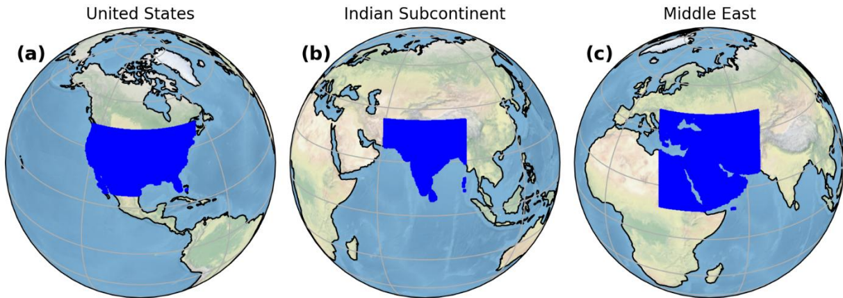
Figure 2. a) Highlighted in a bright blue color are the selected grid regions (each grid is 25x25 km 2 equal) for the USA region. b) Similar to a) but for the Indian Subcontinent (SC) region. c) Similar to a) but for the Middle East region.
