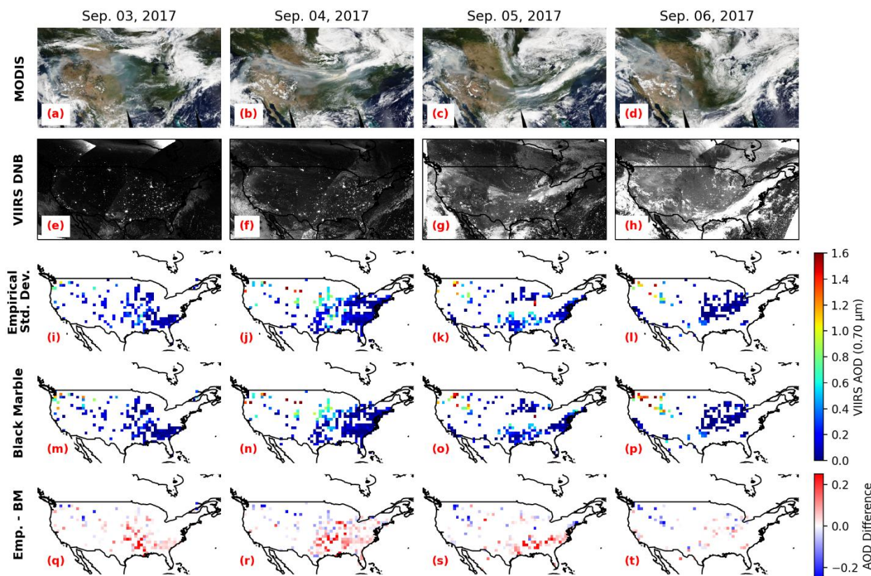
555 Figure 10. a - d) Aqua MODIS true color images over USA for Sep. 03- Sep. 06, 2017. The MODIS true color images were obtained from the NASA Worldview website ( https://worldview.earthdata.nasa.gov ). e - h) Suomi-NPP VIIRS/DNB imagery over the USA for Sep. 03 - Sep. 06, 2017. i - l) Similar to e-h) but for VIIRS/DNB nighttime AOT retrievals derived using the empirically-based STD method for estimating \Delta I_a values. m - p) Similar to i - l) but for VIIRS/DNB nighttime AOT retrievals derived using the NASA VNP46 data for estimating \Delta I_a values. q - t) Similar to m - p), but showing the differences between the nighttime AOT from the 560 empirically-based STD method and the VIIRS/DNB nighttime AOT retrievals.
