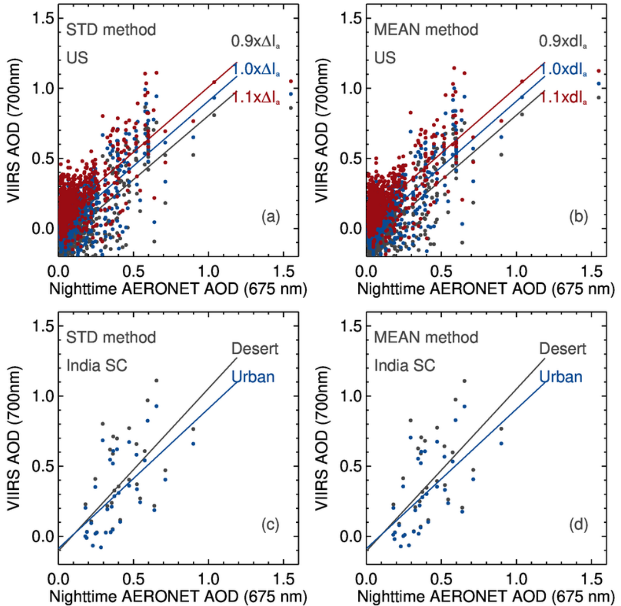
Figure 7. a) Scatter plot of lunar AERONET and VIIRS/DNB AOT as a function of \Delta I_a value for the USA region using the empirically-based STD method. b) Scatter plot of lunar AERONET and VIIRS/DNB AOT as a function of \Delta I_a value for the USA region using the empirically-based Mean method. c) Scatter plot of lunar AERONET and VIIRS/DNB AOT (derived using the empirically-based STD method) over the Indian Subcontinent region using different aerosol models. d) Similar to c) but with the use of the empirically-based Mean method.
