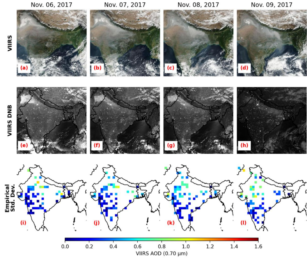
Figure 12. a - d) Suomi-NPP VIIRS true color images over the Indian Subcontinent for Nov. 06 - Nov. 09, 2017, obtained from the NASA Worldview website ( https://worldview.earthdata.nasa.gov/ ; ©NASA). e – h) Suomi-NPP VIIRS/DNB imagery over the Indian
