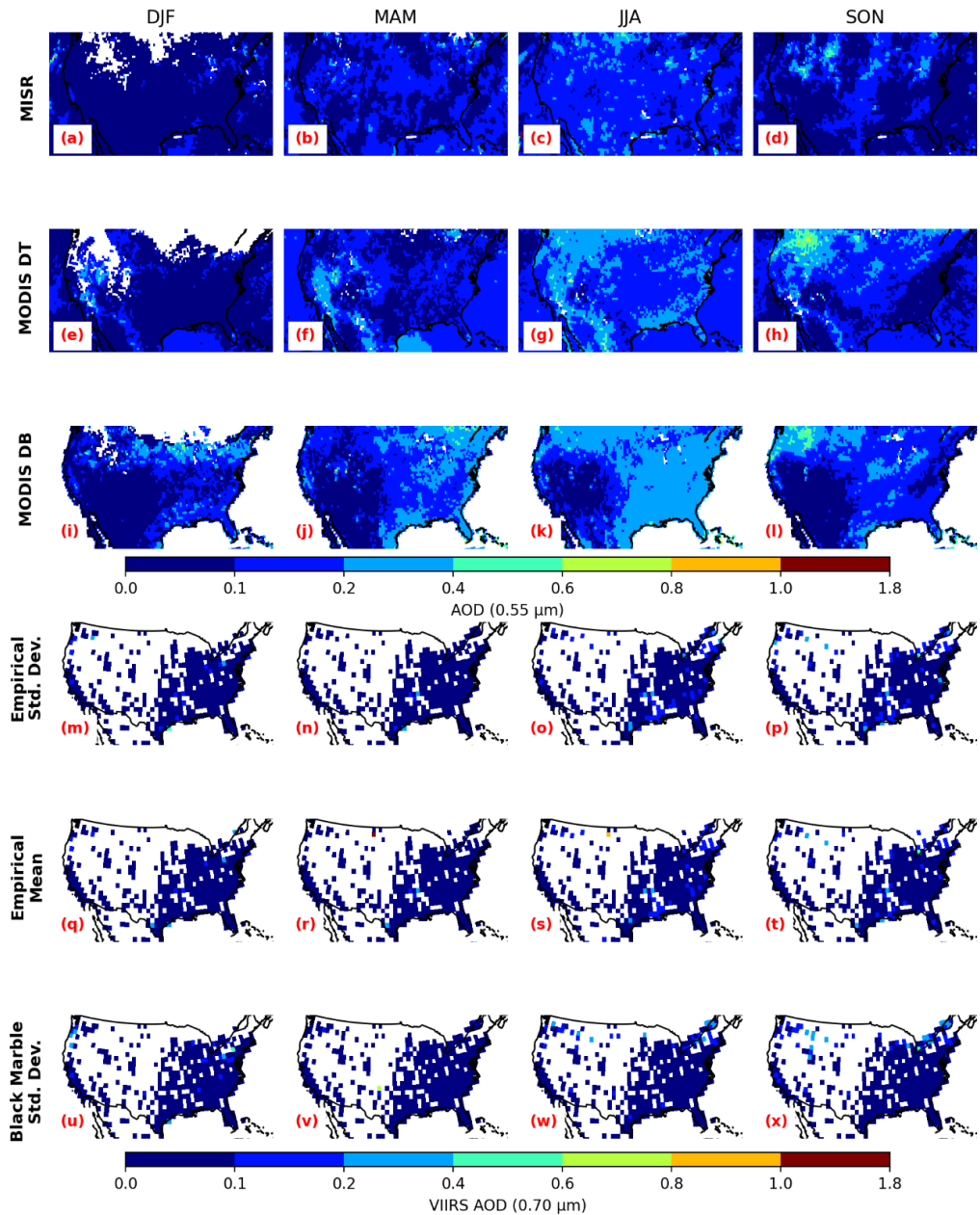
Figure 9. a - d). Seasonally averaged daytime MISR AOT (550nm) over the USA region for the DJF, MAM, JJA, and SON seasons. 525 e - h) Similar to a - d), but for MODIS Dark Target (DT) AOT (550 nm). i - l) Similar to e - h), but for MODIS Deep Blue (DB)
