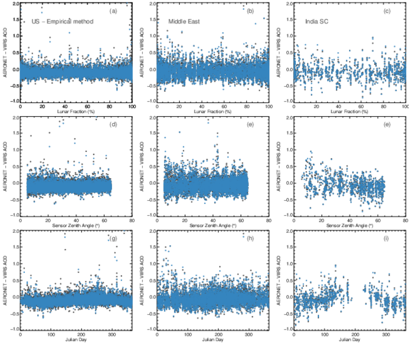
Figure 8. a) The difference between daytime AERONET (675 nm) and nighttime VIIRS/DNB (700 nm) AOT as a function of lunar fraction (%) for the USA region using the empirically-based STD (black color) and mean (blue) colors. d) Similar to a) but showing the difference between daytime AERONET (675 nm) and nighttime VIIRS/DNB (700 nm) AOT as a function of sensor viewing zenith angle. g) Similar to a) but showing the difference between daytime AERONET (675 nm) and nighttime VIIRS/DNB (700 nm) AOT as a function of Julian day. b, e, and h) Similar to a, d and g) but for the Middle East region. c, e and i) Similar to a, d and g), but for the Indian Subcontinent region.
