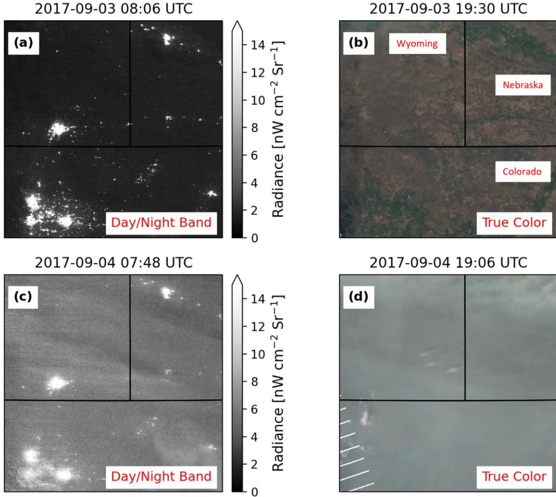
190 Figure 1. a) VIIRS DNB image at 08:06 UTC on Sep. 03, 2017 over Central US. b) VIIRS true color image at 19:30 UTC on Sep. 03, 2017 for the same region as a). Both panels a) and b) correspond to relatively low aerosol loading in the scene. c) Similar to a) but 195 for the VIIRS DNB image at 07:48 UTC on Sep. 04, 2017. d) Similar to b) but for the VIIRS true color image at 19:06 UTC on Sep. 04, 2017. Both panels c) and d) correspond to relatively high aerosol loading (here, biomass smoke) in the scene, with commensurate blurring of city light structures when comparing c) to a). In both the clean and turbid DNB imagery examples, the Moon's phase is in waxing gibbous. Figures were obtained from the NASA Worldview website ( https://worldview.earthdata.nasa.gov/ ; ©NASA)
