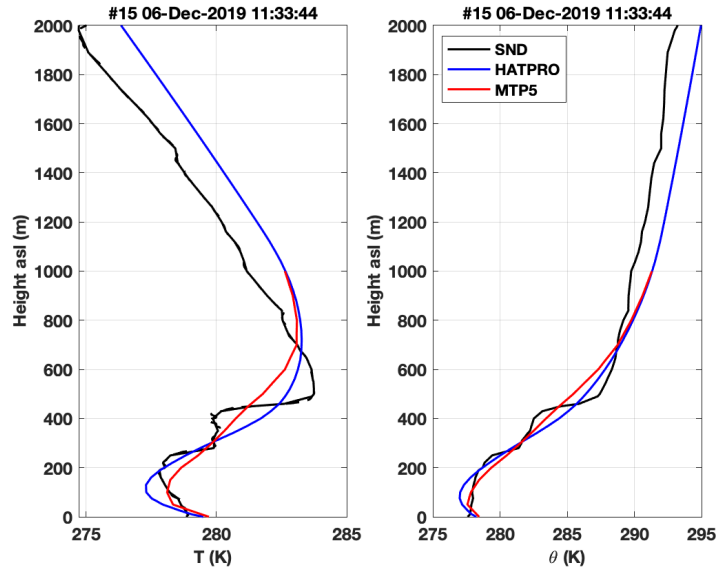
Figure 8: Simultaneous temperature (left) and potential temperature (right) profiles from radiosonde (black) and three MWR types. Top: MP3000-A (red) at the ENA site (unstable conditions). Bottom: HATPRO (blue) and MTP5 (red) at the SOFOG3D supersite (neutral to stable conditions). Note that MTP5 retrievals are limited to 1-km height.
