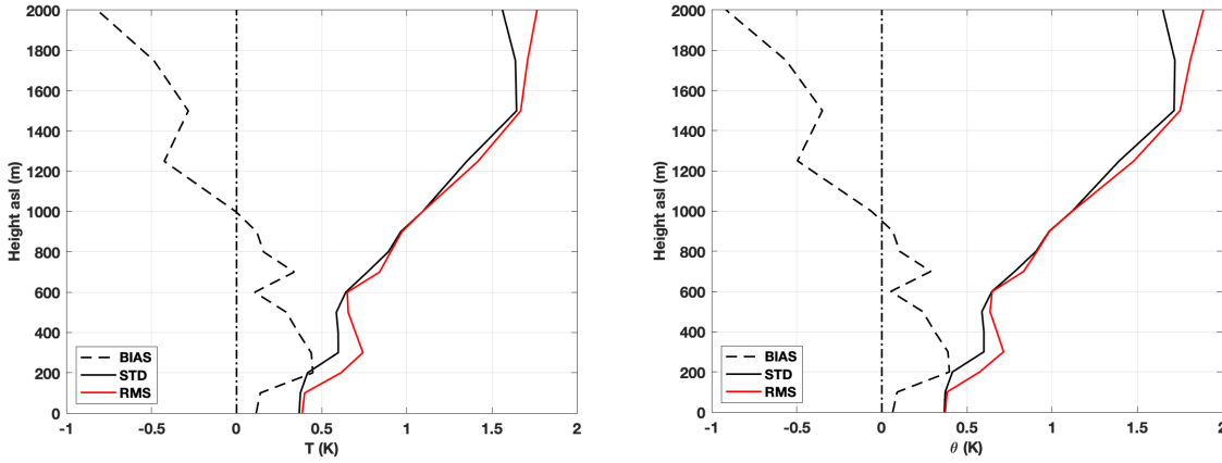
Figure 10: (Left) Bias, standard deviation (STD), and root-mean-square (RMS) differences of the MWR-minus-radiosonde temperature residuals from the 138 matchups collected at the ENA observatory on Graciosa Island (Eastern North Atlantic) from 2019-01-01 to 2019-03-15. (Right) Same but for potential temperature profiles.
