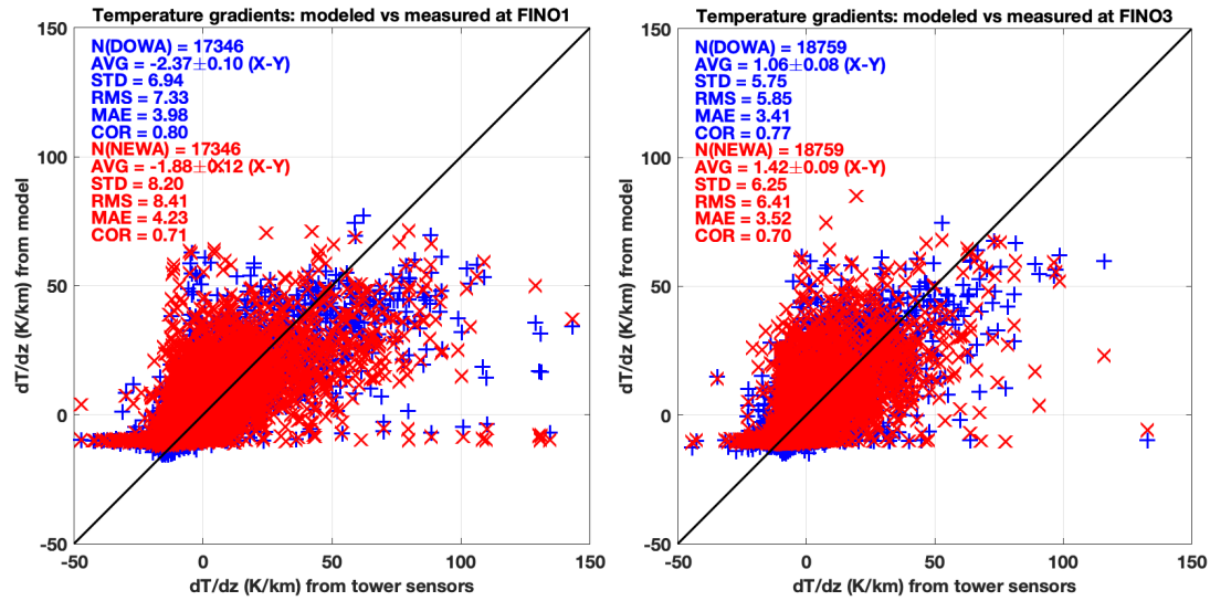
Figure 5. Scatter plots of atmospheric temperature lapse rate ( \sim 50\text{--}100 m) from tower measurements at FINO1 (left) and FINO3 (right) and model data (DOWA: blue crosses; NEWA: red Xs). N indicates the sample size, AVG the average difference ( \pm 95\% confidence interval), STD the standard deviation, RMS the root-mean-square, MAE the mean absolute error, and COR the correlation coefficient R . Units for AVG, STD, RMS, and MAE are in K/km.
