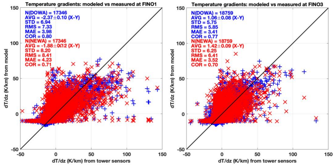
Figure 5. Scatter plots of atmospheric temperature lapse rate ( \sim 50 – 100 m) from tower measurements at FINO1 (left) and FINO3 (right) and model data (DOWA: blue crosses; NEWA: red Xs). N indicates the sample size, AVG the average difference ( \pm 95\% confidence interval), STD the standard deviation, RMS the root-mean-square, MAE the mean absolute error, and COR the correlation coefficient R . Units for AVG, STD, RMS, and MAE are in K/km.
