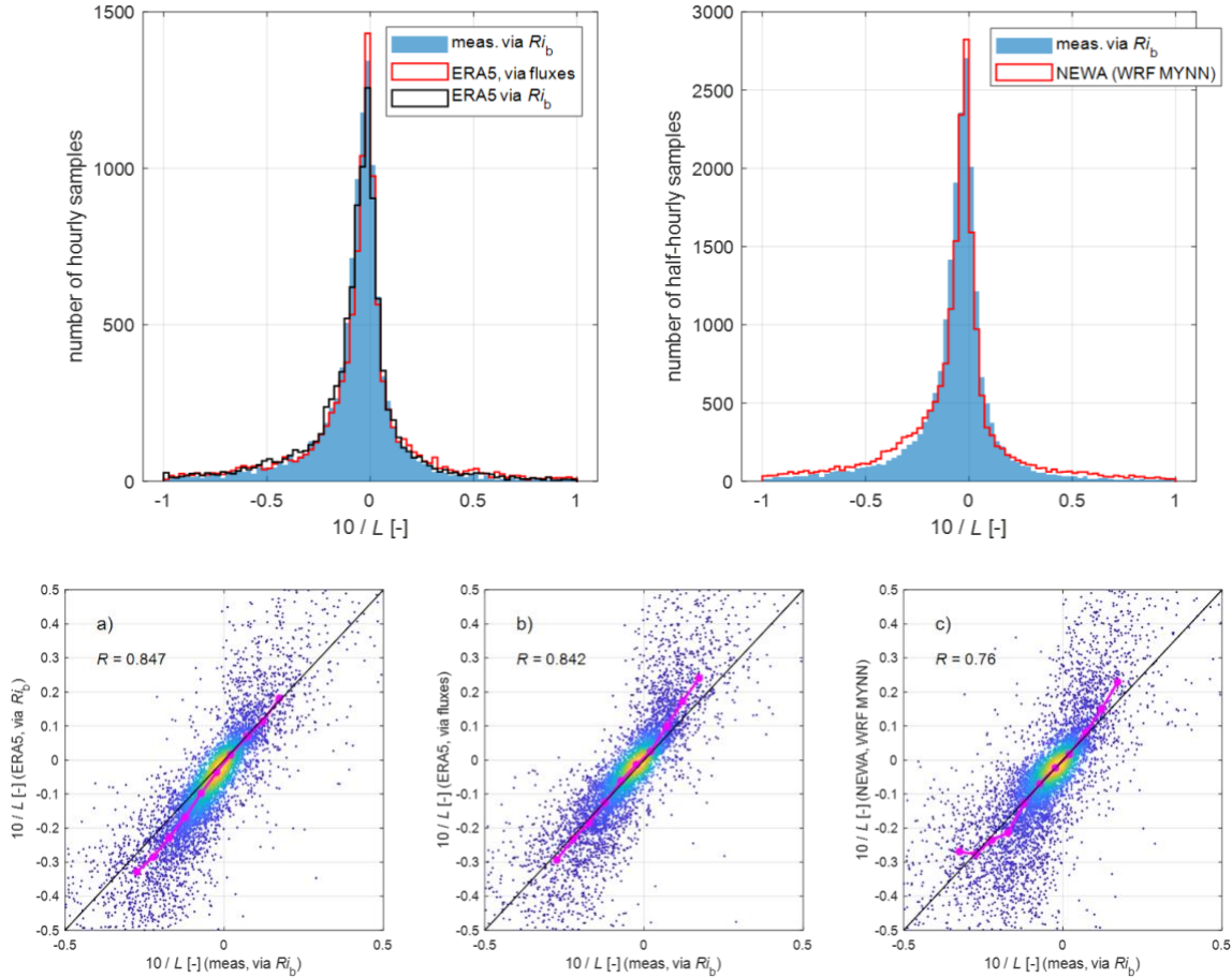
Figure 1. Comparison of measurements ( R_b -based) and NWP model data of the dimensionless stability parameter z/L (where z = 10 m ASL and L is the Obukhov length) at the HKZA floating lidar location. Top: Histograms of z/L . The same measurements are sampled hourly to compare with ERA5 (left) and half-hourly to compare with NEWA (right) data. Bottom: Scatter plot of hourly averaged measurements vs. ERA5 (a and b, for R_b - and fluxes-based, respectively) and NEWA (c) model data, for 10 m ASL wind speeds larger than 10 m/s. R indicates the correlation coefficients between the model and measurements time series, while the magenta line shows binned mean values.
