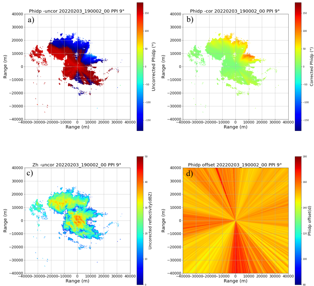
Fig. C1: PPI at an elevation of 9^\circ at 19 UTC on February 3, 2022: (a) raw differential phase shift, (b) corrected \Phi DP (using the procedure described in this article), (c) raw reflectivity, and (d) system offset illustrating its variation along the azimuth.
