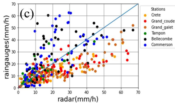
450 Figure 8: Radar quantitative precipitation estimation using a) R(Z) estimator and Hitschfeld and Bordan attenuation correction; b) R(Z) estimator and \phi -linear attenuation correction; c) R(kdp) estimator
