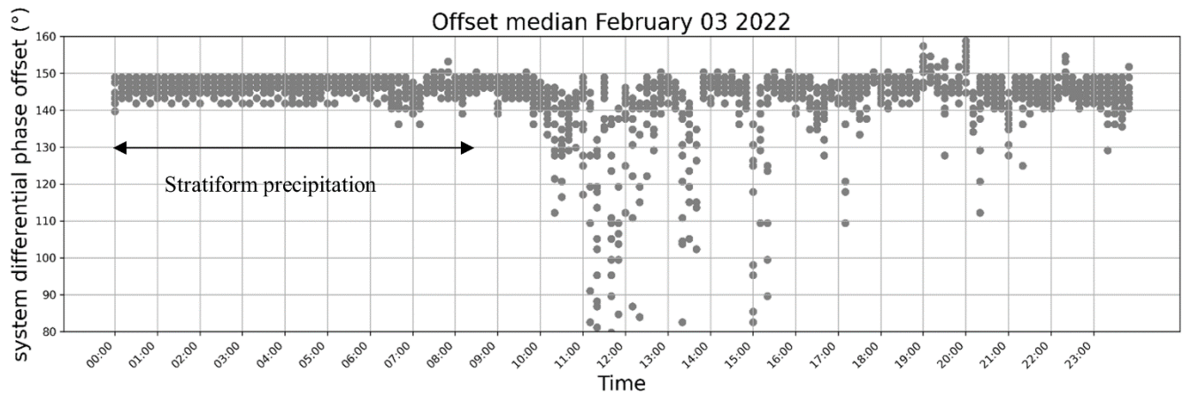
325 Figure 4: Median of system differential phase offset for each scan and timestep on February 3, 2022 the period when the cyclone was close to Reunion Island (~190km from the north coast). During this period two types of precipitation were identified, stratiform precipitation from 00:00 to 8:40 UTC then the precipitation became heavy and characterized by convective rain.
