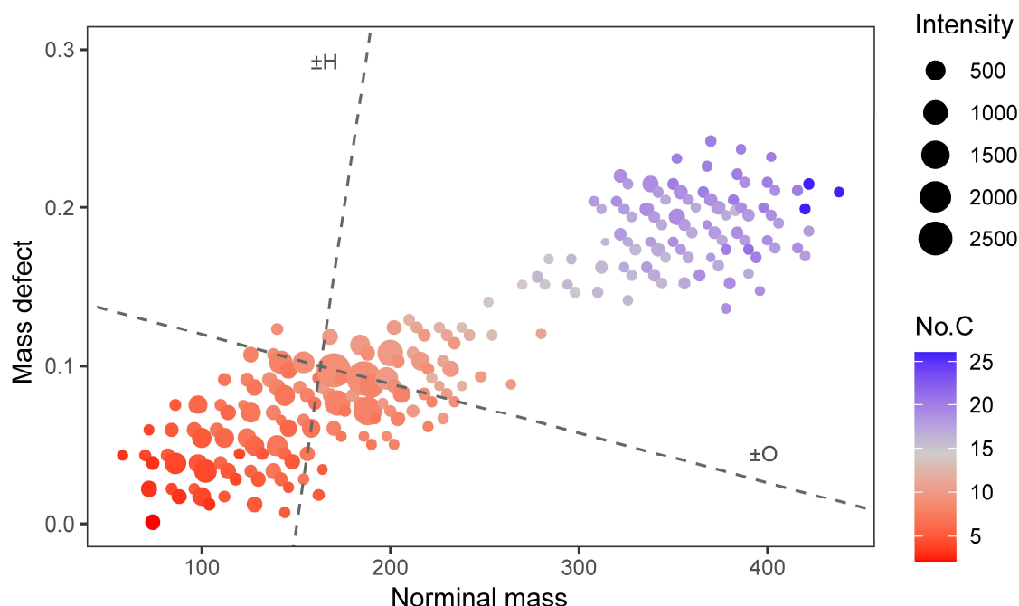
Figure 6. The mass defect plot of the ozonolysis products in the fast \alpha -pinene injection experiment. The data in the figure correspond to the moment when the particle mass concentration peaked. Dash lines in the figure represent the changes in mass defect when an oxygen (O) or hydrogen (H) atom was added to a compound. The addition of an H atom will increase the mass defect while the addition of an O atom will decrease the mass defect of a compound.
