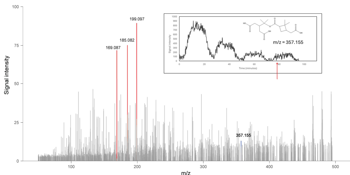
360 Figure 8. Mass spectrum of products during the no-filter phase in the fourth rotation cycle in slow \alpha -pinene injection experiment. Peaks with signal intensity larger than 50 were highlighted in red. The plot embedded in the mass spectrum corresponds to the time profile of a dimeric product with m/z = 357.155 . The red arrow in the plot corresponds to the time when the mass spectrum is obtained.
