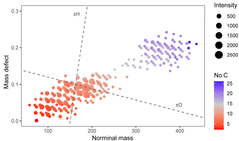
Figure 6. The mass defect plot of the ozonolysis products in the fast \alpha -pinene injection experiment. The data in the figure correspond to the moment when the particle mass concentration peaked. Dash lines in the figure represent the changes in mass defect when an
