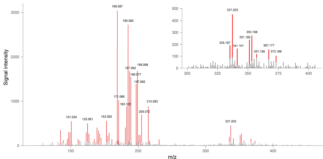
280 Figure 5. The mass spectrum obtained from the fast \alpha -pinene injection experiment when the particle mass concentration was the highest. The mass spectrum is background subtracted. Peaks with signal intensity larger than 100 are highlighted in red, and the m/z for peaks with signal intensity larger than 450 are labelled in the figure. The upper right panel shows the magnification of the m/z = 300 to 400 range of the same mass spectrum. Peaks with signal intensity larger than 100 are highlighted in red and labelled with their corresponding m/z .
