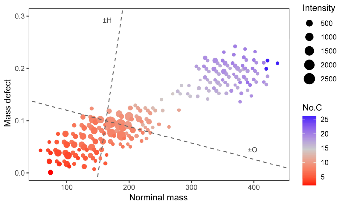
285 Figure 6. The mass defect plot of the ozonolysis products in the fast \alpha -pinene injection experiment. The data in the figure correspond to the moment when the particle mass concentration peaked. Dash lines in the figure represent the changes in mass defect when an
