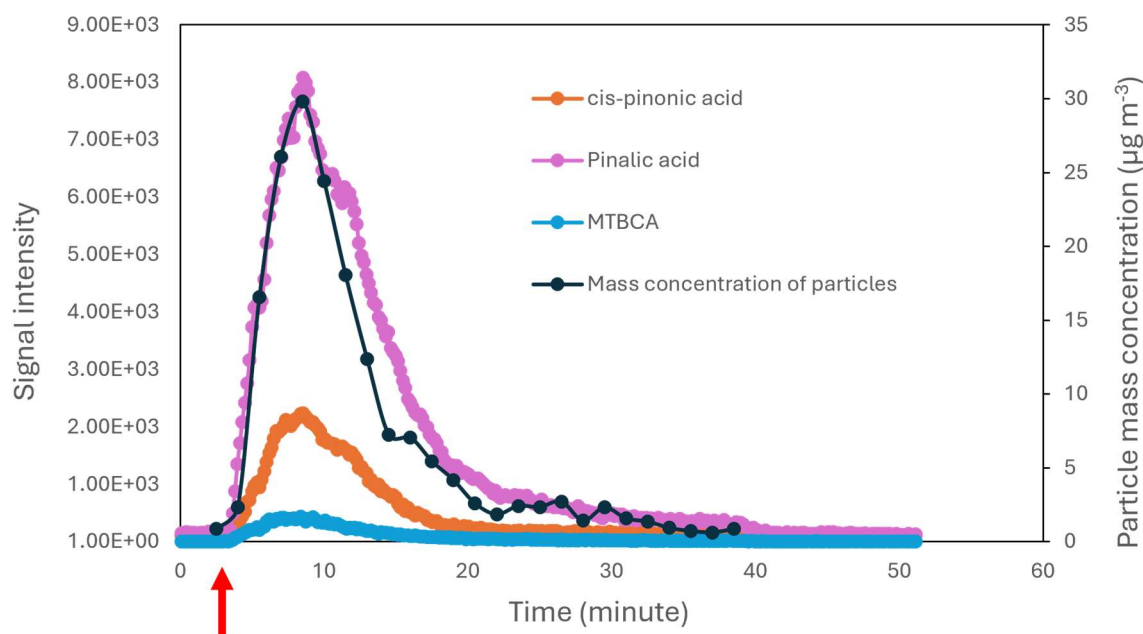
265 Figure 4. The mass concentration of particles measured by the SMPS and the signal intensity of selected \alpha -pinene ozonolysis products captured by the ESI-Orbitrap-MS for the fast \alpha -pinene ozonolysis experiment. The red arrow marks the injection time of \alpha -pinene.
