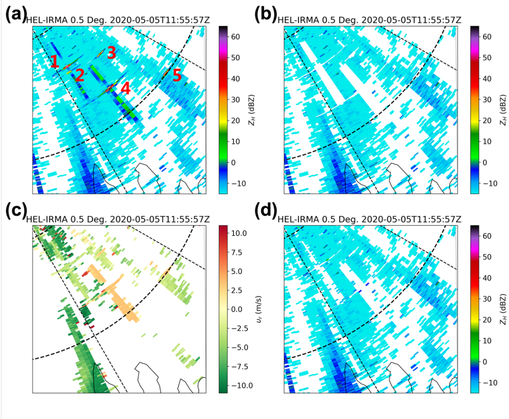
Figure 8: 0.5° elevation of Kumpula radar using LFM waveform at 1155 UTC 5 May 2020. (a) Reflectivity before ship-clutter filtering; (b) Reflectivity after filtering all range gates in the PSD; (c) Doppler velocity; (d) Reflectivity after filtering using velocity and SNR thresholds.
