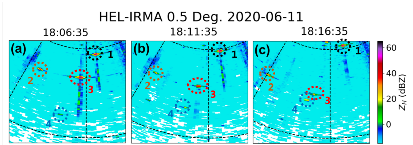
Figure 4: Typical ship clutter observed by Kumpula radar at (a) 1806 UTC, (b) 1811 UTC, and (c) 1816 UTC on 11 June 2020. Dashed circles with different colors indicate ship clutters, respectively.
