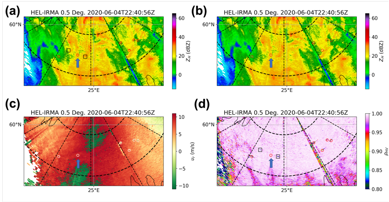
Figure 12: 0.5° elevation of Kumpula radar using LFM waveform at 2240 UTC 4 June 2020. (a) Reflectivity before ship clutter filtering; (b) Reflectivity after ship clutter filtering; (c) Doppler velocity before ship clutter filtering; (d) co-polar correlation coefficient after ship clutter filtering. The mainlobe identification results are highlighted with red or white circles, with misidentified cases indicated by blue arrows, while the unrecognized ones are highlighted with black rectangles.
