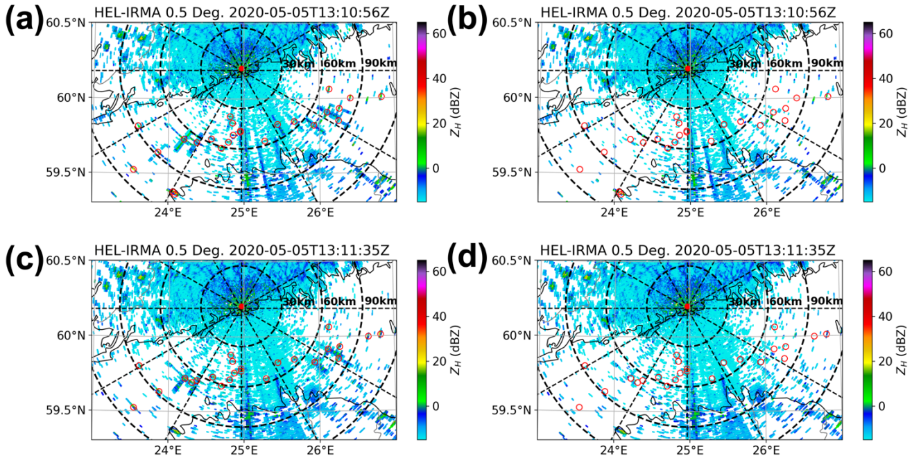
Figure 11. Reflectivity on 0.5° elevation of Kumpula radar using LFM (1310 UTC) and NLFM (1311 UTC) waveforms on 5 May 2020. (a) Before ship clutter filtering using LFM waveform; (b) After ship clutter filtering using LFM waveform; (c) Before ship clutter filtering using NLFM waveform; (d) After ship clutter filtering using NLFM waveform. The mainlobe identification results are highlighted by red circles.
