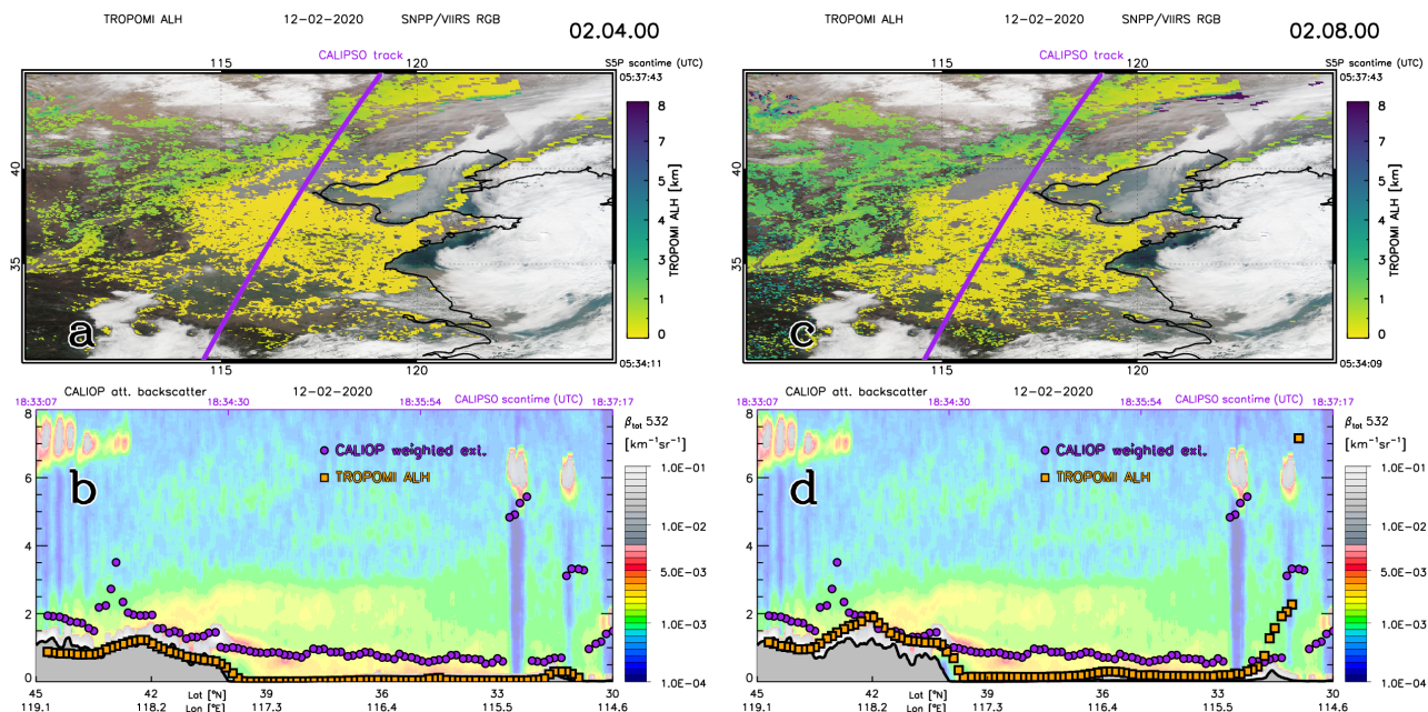
Figure A5. Same as Fig A1, but on 12 Feb. 2020 showing industrial pollution over China, from 5:33:48–5:37:48 UTC for TROPOMI data and 18:33:07–18:37:17 UTC for CALIOP data. Note that CALIOP data were collected from the nighttime overpass in order to get a good coverage of the plume over Beijing.
