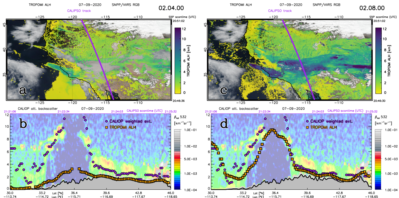
Figure 2. (a) True color (RGB) image from SNPP/VIIIRS on 7 Sept. 2020 showing Californian smoke plumes over north-west America, overlaid with TROPOMI ALH, version 02.04.00 from 20:46:36–20:51:02 UTC. The purple line shows the daytime CALIPSO track over the area on the same day from 21:21:06–21:25:32 UTC. (b) CALIOP L1 532 nm attenuated backscatter curtain image along the purple track in the top panels, overlaid with the CALIOP weighted extinction height (purple dots) from L2 extinction profiles at 532 nm (averaged every 0.15^\circ latitude along the track) and the average TROPOMI ALH of collocated pixels within a 0.5^\circ radius of the CALIOP extinction profiles along the track. Note that ALH is given from sea level, so retrievals at the ground over an elevated surface are not necessarily zero. Elevated surfaces are grey shaded in the bottom curtain plots. (c) and (d): Same as (a) and (b) respectively, but with TROPOMI ALH version 02.08.00.
