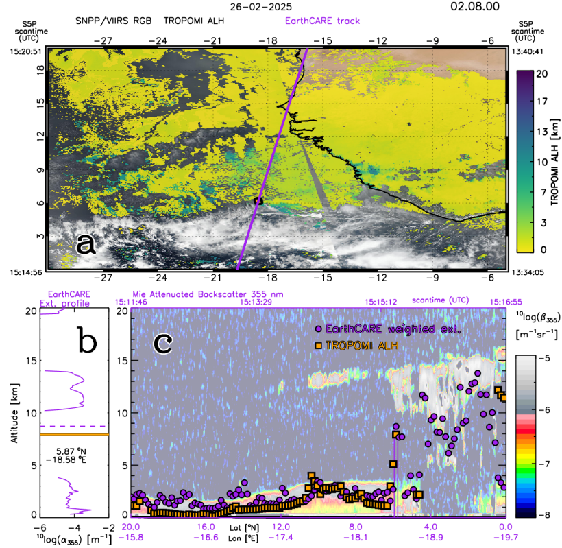
Figure 6. (a) True color (RGB) image from SNPP/VIIIRS on 26 Feb. 2025 showing a desert dust outbreak over the Sahel and north-east Atlantic Ocean, overlaid with TROPOMI ALH, version 02.08.00 from 13:34:05–13:40:41 UTC (covering the right part of the image) and from 15:14:56–15:20:51 UTC (covering the left part of the image). The purple line shows the daytime EarthCARE track over the area on the same day from 15:11:46–15:16:55 UTC. Note that during daytime, EarthCARE is in a descending orbit, while Sentinel-5P is in an ascending orbit. The orange-black dot shows the location of the profile in panel (b); (b) ATLID L2 extinction profile at 335 nm at 5.9°N, -18.6°E (solid purple line), weighted extinction height of this ATLID profile (dashed purple line) and the TROPOMI ALH at this location (orange-black line); (c) ATLID L1 335 nm mie attenuated backscatter curtain image along the purple track in the top panel, overlaid with the ATLID weighted extinction height (purple dots) from L2 extinction profiles at 335 nm (averaged every 0.15° latitude along the track) and the average TROPOMI ALH of collocated pixels within a 0.5° radius of the ATLID extinction profiles along the track. The location of the profile in (b) is indicated by vertical purple lines.
