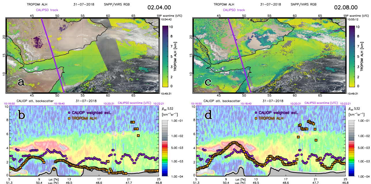
Figure 4. (a) True color (RGB) image from SNPP/VIIIRS on 31 Jul. 2018 showing a dust plume over the Arabian Peninsula, overlaid with TROPOMI ALH, version 02.04.00 from 10:49:31–10:55:12 UTC. The purple line shows the daytime CALIPSO track over the area on the same day from 10:16:50–10:22:21 UTC. (b) CALIOP L1 532 nm attenuated backscatter curtain image along the purple track in the top panels, overlaid with the CALIOP weighted extinction height (purple dots) from L2 extinction profiles at 532 nm (averaged every 0.15° along the track) and the average TROPOMI ALH of collocated pixels within a 0.5° radius of the CALIOP extinction profiles along the track. (c) and (d): Same as (a) and (b), but with TROPOMI ALH version 02.08.00.
