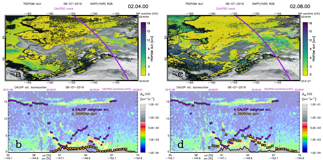
Figure A4. Same as Fig A1, but on 8 July 2019, showing multiple layers of biomass burning smoke over Alaska, from 22:41:13–22:43:07 UTC for TROPOMI data and 22:31:30–22:35:51 UTC for CALIOP data. CALIOP weighted extinction heights are found at around 15 km altitude around 56°N which coincides with a peak in the L1 backscatter coefficient due to a high altitude layer of smoke. The TROPOMI ALH is cloud-screened at those latitudes. TROPOMI ALH is found around 1–5 km altitude between 60–70°N, which coincides with a peak in the L1 backscatter coefficient due to a low altitude layer of smoke. CALIOP weighted extinction heights are found at intermediate heights between these high and low altitude layers.
