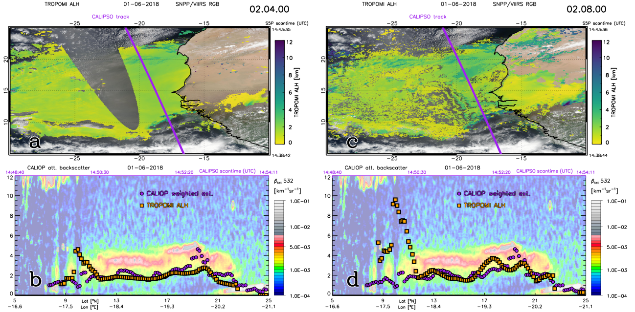
Figure A1. (a) True color (RGB) image from SNPP/VIIIRS on 1 June 2018 showing a dust plume over the Sahara desert and the northeast Atlantic Ocean, overlaid with TROPOMI ALH, version 02.04.00 from 14:37:59–14:43:35 UTC. The purple line shows the daytime CALIPSO track over the area on the same day from 14:48:40–14:54:11 UTC. (b) CALIOP L1 532 nm attenuated backscatter curtain image along the purple track in the top panels, overlaid with the CALIOP weighted extinction height (purple dots) from L2 extinction profiles at 532 nm (averaged every 0.15^\circ latitude along the track) and the average TROPOMI ALH of collocated pixels within a 0.5^\circ radius of the CALIOP extinction profiles along the track. (c) and (d): Same as (a) and (b), but with TROPOMI ALH version 02.08.00.
