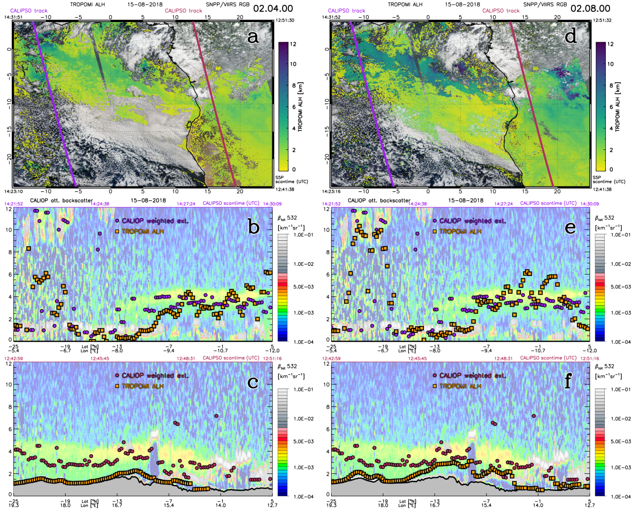
Figure A2. Same as Fig A1, but on 15 Aug. 2018 showing biomass burning smoke during two overpasses, the southeast Atlantic ocean from 14:23:52–14:31:51 UTC for TROPOMI data and 14:21:52–14:30:09 UTC for CALIOP data, and over central African and from 12:41:52–12:50:17 UTC for TROPOMI data and 12:42:59–12:51:16 UTC for CALIOP data.
