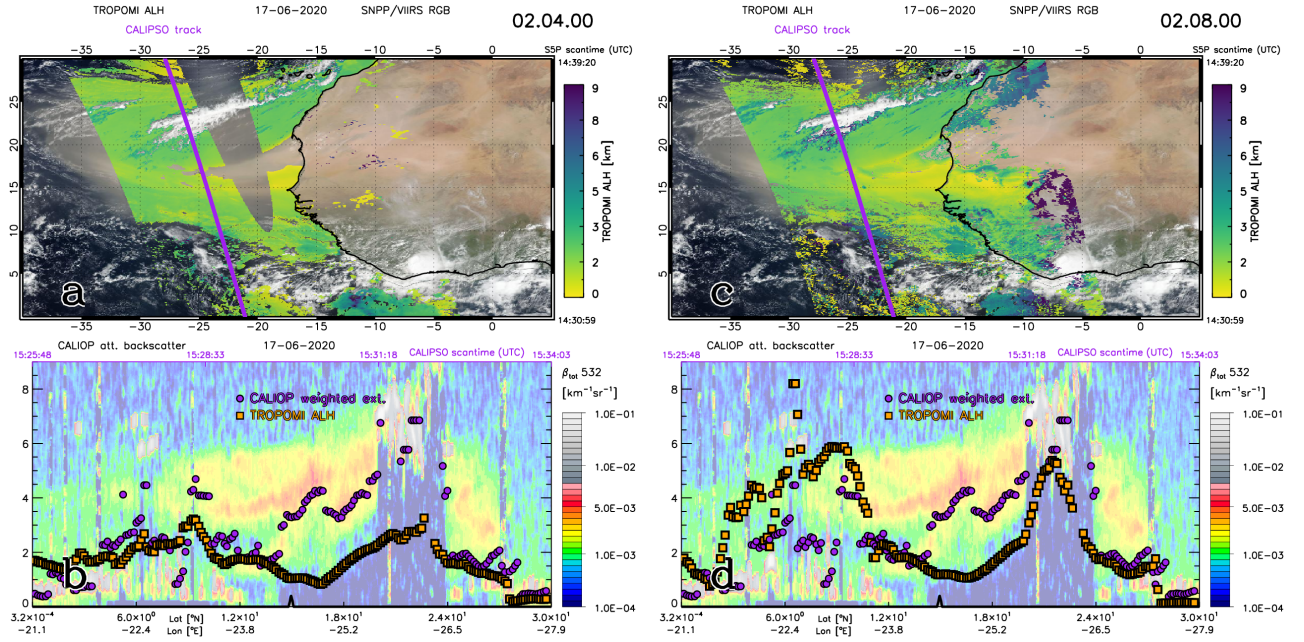
Figure A6. Same as Fig A1, but on 17 June 2020 from 14:30:58–14:39:20 UTC for TROPOMI data and 15:25:48–15:34:03 UTC for CALIPSO data.
