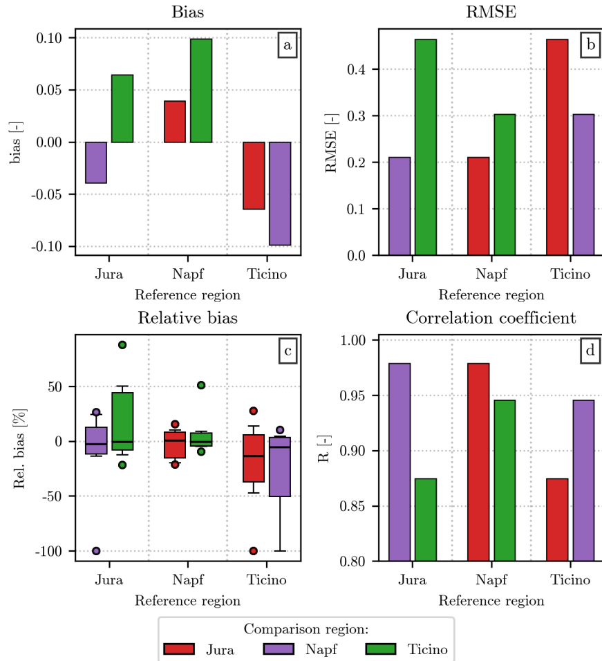
Figure 7. Comparison of the median value of h(x) between the three regions of deployment of the hail sensors. Similarly to Figure 3, the values of bias (panel a), RMSE (panel b), and \text{PCC}_R (panel d) are indicated by the height of the vertical bars, while the information on the distribution of the relative bias (panel c) is provided in the form of boxplots. As in Figure 6, the reference region for h(x) is shown on the x-axis, while the color of the bars/boxplots shows the region to which it is compared.
