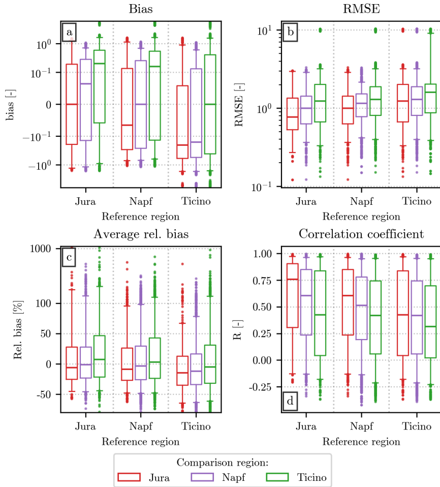
Figure 6. Comparison of the normalized distributions from all the events recorded in each of the three regions of deployment of the hail sensors. The comparison is always performed between all possible combination of pairs of events, one of which belongs to a reference region shown on the x-axis, while the region of the second one is shown by the line colors and the position of the boxplot: red for the Jura (leftmost one), purple for Napf (central one), and green for Ticino (on the right). All combinations of different events have been used for the computation of the error metrics. The order in which these error metrics have been assigned to different panels and the structure of the individual boxplots is analogous to the one in Figure 5. The scale of the y-axis in panel a and d is linear inside the intervals [-0.1, 0.1] and [-100, 100] , respectively, and logarithmic outside of them.
