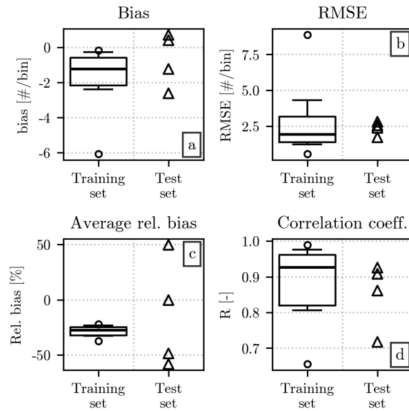
Figure 12. As Figure 11, but using only the values N_u(D) and \hat{N}_u(D) for diameters above 10 mm. Measurements for at least 5-five discrete diameter values have to be present in each event for it to be included in the comparison. Due to the scarcity of such events in the test set, the values of the error metrics for each of them are displayed individually as triangular markers.
