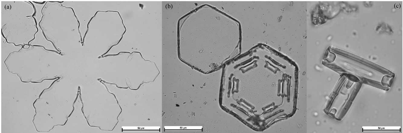
180 Figure 3. Optical microscope images of random crystal with a shape of: (a) stellar plate, (b) hexagon and (c) column.
