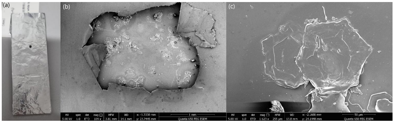
Figure 4. SEM imaging steps described: (a) sample 73 covered with foil with an opening in it, (b) the selected area's SEM image and (c) close-up image of two hexagonal plates that overlap.
