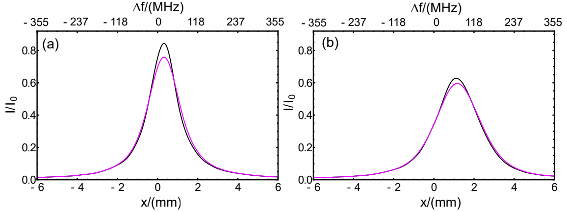
Figure 10. Fringe profiles modelled before (black) and after (magenta) convolution with a Gaussian laser pulse profile of 45 MHz FWHM. (a): AOI = -100 \mu\text{rad} , FOV = 500 \mu\text{rad} . (b): AOI = +300 \mu\text{rad} , FOV = 500 \mu\text{rad} .
