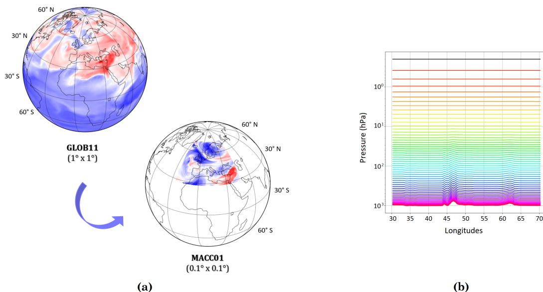
Figure 4. (a) Illustration of MOCAGE global domain GLOB11, which presents a 1^\circ \text{lat} \times 1^\circ \text{lon} horizontal resolution, and the regional domain over Europe, named MACC01, with a thinner resolution of 0.1^\circ \text{lat} \times 0.1^\circ \text{lon} , and bounded in 28^\circ \text{N} , 26^\circ \text{W} and 72^\circ \text{N} , 46^\circ \text{E} . Colors indicate ozone field at a given level. (b) [adapted from El Aabaribaoune (2022)] MOCAGE vertical configuration of the 60 hybrid \sigma -pressure levels (each one represented with a different colour).
