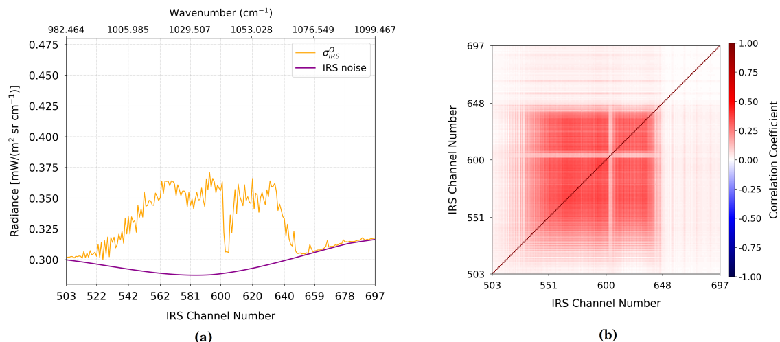
Figure 10. Diagnosed observation-error standard deviations ( \sigma_{IRS}^O ) and instrument noise for IRS in (a) and diagnosed error correlations in (b).
