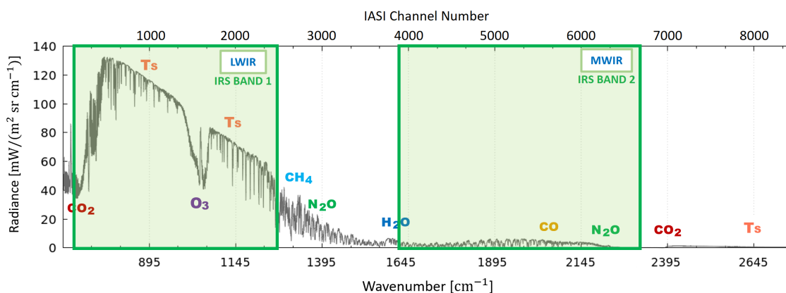
Figure 2. The two bands that IRS will cover are here highlighted in green on the infrared spectrum covered by IASI (in radiance units). Band 1 in LWIR goes from 679.70 to 1210.44 cm -1 , while band 2 in the MWIR is bounded in 1600.00 – 2250.20 cm -1 . Sensitivities to different species are also highlighted (Ts means surface temperature).
