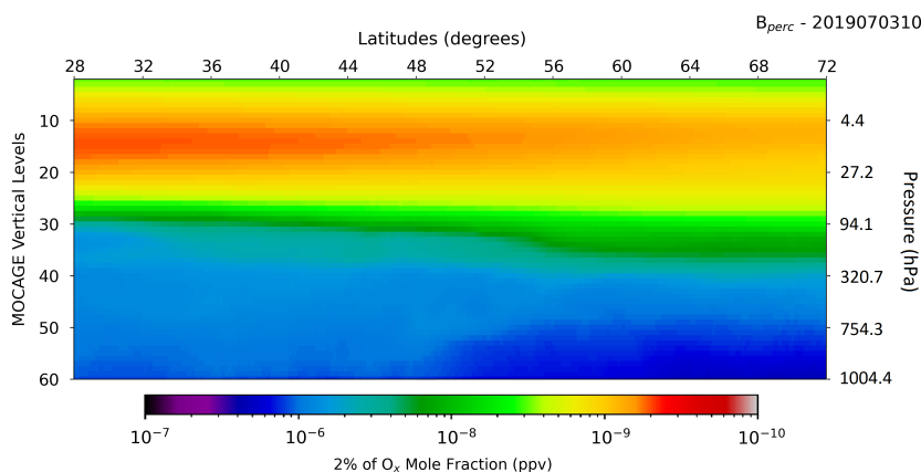
Figure 11. Example of B matrix, obtained as 2% of the ozone concentration, for one random day and hour inside the period of study (3rd of July, 2019, 10 UTC). Values are averaged over longitudes.
