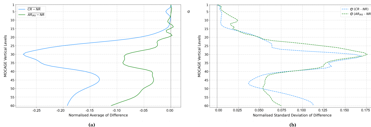
Figure 14. Normalised average (a) and standard deviation (b) of differences between CR and NR in blue (rp. AR for IRS and NR in green). The normalization is done with the average NR profile. The statistics are computed, for each MOCAGE vertical level, over the 3-month period of study (1st of June up to 31st of August, 2019) and the geographical MACC01 domain.
