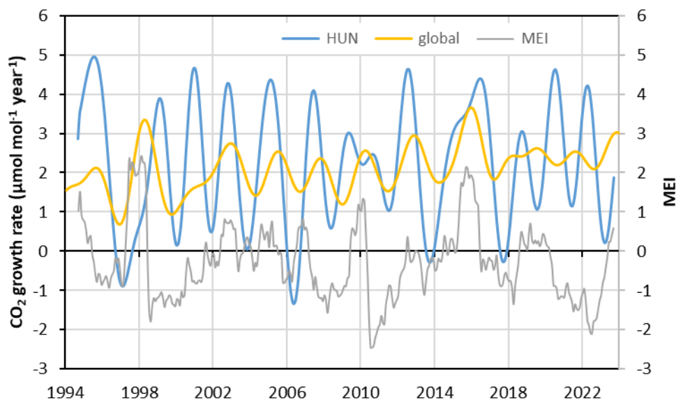
485 Figure 12: The temporal variation of the growth rate of CO 2 concentration at 115 m elevation at Hegyhátsál (HUN) and in the global atmosphere, as well as that of the Multivariate ENSO index (MEI). The global growth rate has been calculated from the globally averaged marine surface monthly mean data ( https://gml.noaa.gov/webdata/ccgg/trends/co2/co2_mm_gl.txt – accessed on 27 May 2024).
