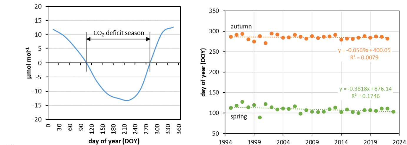
Figure 9: Temporal variations of the beginning and end of the CO 2 deficit season, the spring and autumn zero-crossings at 115 m above the ground.
