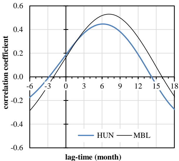
510 Figure 13: Correlation coefficient between the CO 2 growth rate and the Multivariate ENSO Index at Hegyhátsál (HUN) and in the marine boundary layer as the functions of the lag-time.
