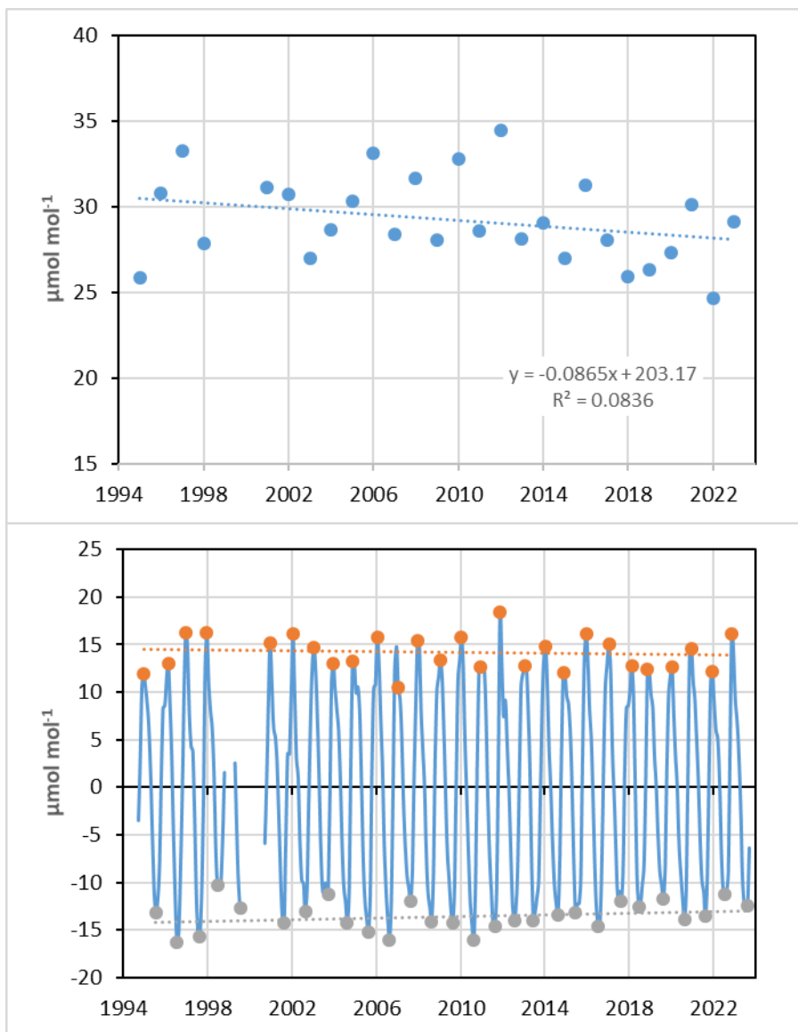
450 Figure 10: Temporal variation of the seasonal amplitude at Hegyhátsál at 115 m elevation (upper panel), and the tendencies in summer (April-September) minimums and winter (October-March) maximums. 1999-2000 was not taken into account in the trend estimations due to the repeated and prolonged data gaps caused by technical problems.
