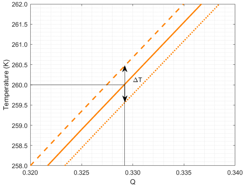
185 Figure 8. Like Fig. 7 with the filters of Fig. 2 shifted 8.57\text{ cm}^{-1} towards shorter wavelengths.
