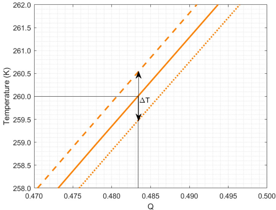
165 Figure 7. Example of uncertainty in the temperature retrieval ( \Delta T ) due to the uncertainty in the laser central wavelength. Solid curve: assumed calibrated Q obtained as the ratio between the output powers of the IF3 (orange) filter and the IF1 (blue) filter of Fig. 1 at the 354.7133 nm wavelength; dashed and dotted curves: Q obtained for wavelength deviations with respect to the calibration wavelength of +1.5 pm and -1.5 pm respectively. Note that the axes are swapped with respect to those in Fig. 6 to emphasize that Q is the variable from which the temperature is retrieved.
