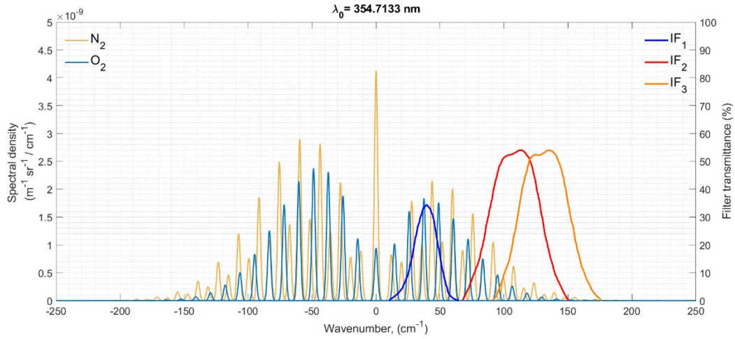
90 Figure 1. Cabannes lines and pure rotational backscatter Raman spectrum of N 2 (yellow lines) and O 2 (turquoise lines) at sea level under the assumption of a Gaussian-widened excitation at 354.7133 nm. The spectrum is given as wavenumber shift from the excitation wavenumber. The transmission curves of the filters and combination of filters in Hammann et al., 2015 are superimposed, transposing the wavelength scale in that reference to the wavenumber scale here. The filter denoted as IF2 (red transmission curve) is used in high background-radiation situations, whereas the IF3 filter (orange line) is optimized for low background ones. The Cabannes-line amplitudes (zero shift) are divided by 500 to fit them into the graph.
