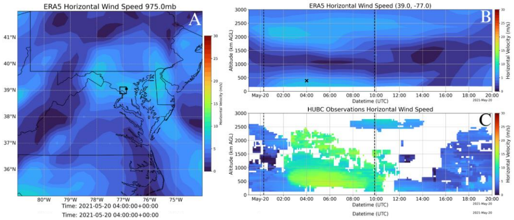
Figure 1- Example depiction of the nocturnal low-level jet in the Mid-Atlantic US on May 20, 2021: (A) ERA5 Horizontal Wind Speed at 975 mb (“x”); (B) shows the vertical-profile evolution of the horizontal-wind speed taken from a vertical slice (black square); (C) shows the horizontal-wind speed from (black circle). Dashed vertical lines indicate the sunset and sunrise times, respectively.
