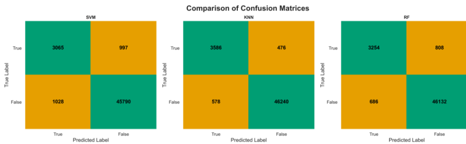
Figure 5: Model training confusion matrices: (green) shows correctly-labelled points by the algorithms while (orange) shows incorrectly-labelled. Top-left indicates true-positive labels, bottom-right indicates true-negative; while bottom-left indicated false-positive, and top-right indicates false-negative.
