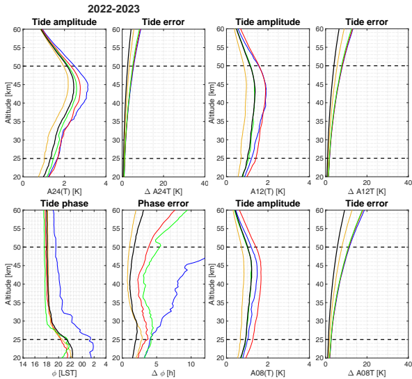
Figure 8. Left: Seasonal averaged diurnal tide amplitude and phase profile with the corresponding tide and phase error (as in Figure 7). Right: Seasonal averaged semi-diurnal and ter-diurnal tide profiles with the corresponding tide error (see section 5).
