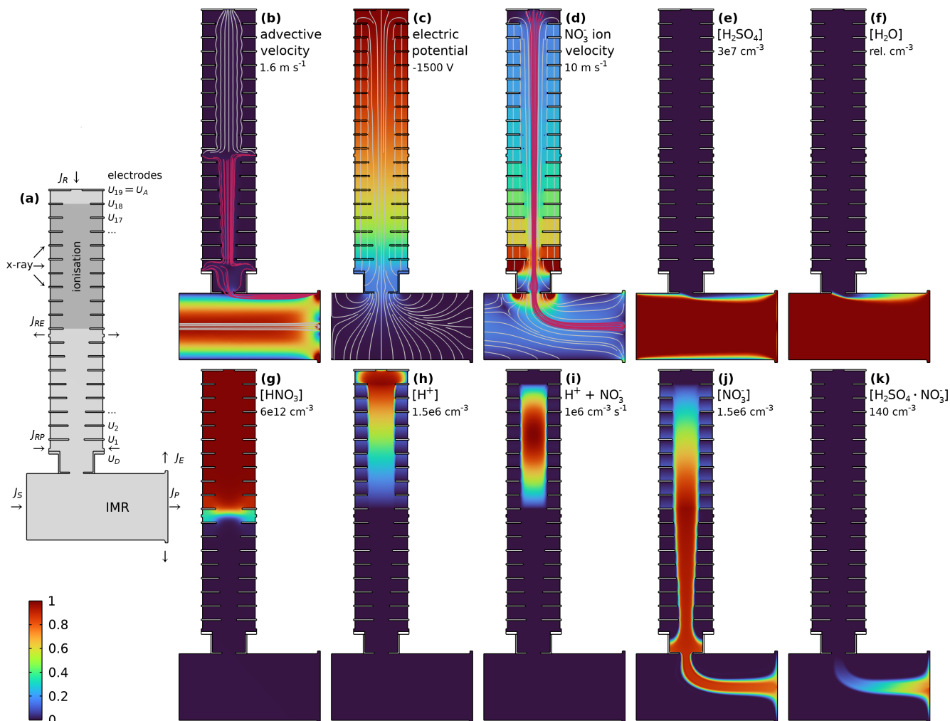
Figure 1. Modelled physical quantities in the MION2 inlet centre plane using \text{NO}_3^- as the reagent ion. The colour scale ranges from 0 to the maximum described in each panel. Panel d shows the electro-advective velocity for anions with \mu = 2.4 \text{ cm}^2 \text{ V}^{-1} \text{ s}^{-1} . Used settings: Accelerator voltage U_A = -1500 \text{ V} , deflector voltage U_D = -110 \text{ V} , exhaust flow J_E = 20 \text{ slpm} , pinhole flow J_P = 800 \text{ sccm} , reagent gas flow J_R = 15 \text{ sccm} , reagent exhaust flow J_{RE} = 50 \text{ sccm} , reagent purge flow J_{RP} = 100 \text{ sccm} .
