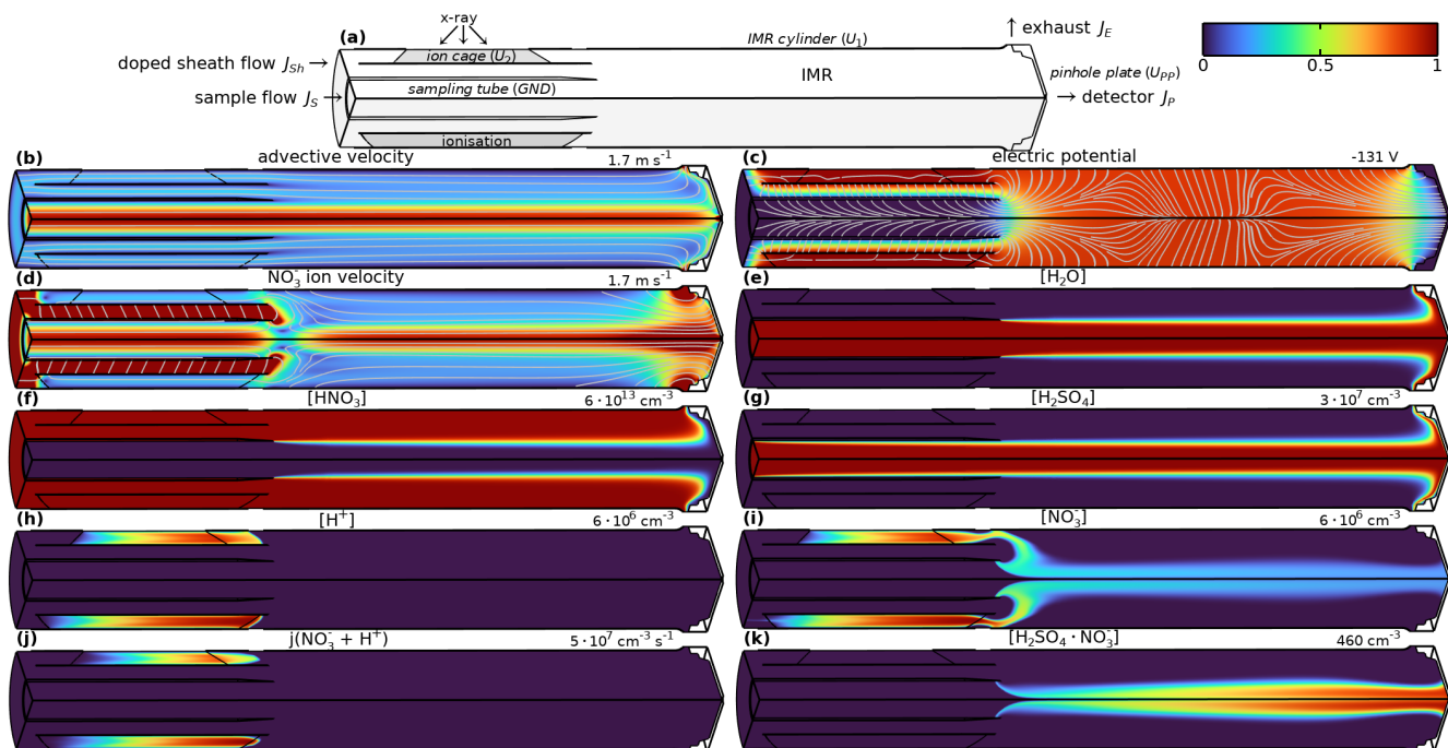
Figure 7. Modelled physical quantities in Eisele type inlet. Only a quarter cut is shown. The colour scale ranges from 0 to the maximum described in each panel. Panel d shows the electro-advective velocity for anions with \mu = 2.4 \text{ cm}^2 \text{ V}^{-1} \text{ s}^{-1} . Used settings: U_1 = -110.7 \text{ V} , U_2 = -98.9 \text{ V} , U_{PP} = 0 \text{ V} , sheath flow 20slpm, sample flow 10slpm.
