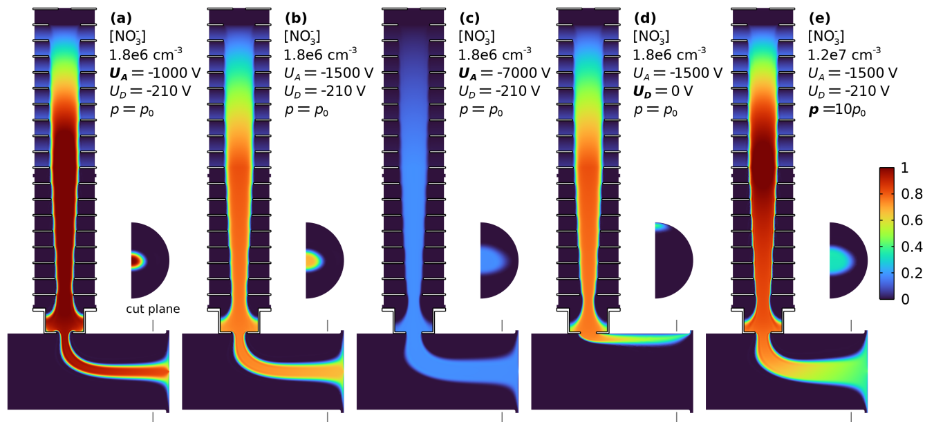
Figure 4. Sensitivities of \text{NO}_3^- concentrations in MION2 inlet to different acceleration voltages U_A (a–c), deflector voltage U_D = 0\text{ V} for deactivation (d), and primary ion production rate (e). The semi circle areas show the ion concentration in the cut plane 5 mm in front of the orifice. The colour scale ranges from 0 to the maximum described in each panel. Figures a–d use the same colour scale. The width of the ion beam increases for larger voltages, while the extracted concentrations slightly decrease. At concentrations of 10^7\text{ cm}^{-3} space charge leads to a spreading of the ion beam, the concentration at the pinhole is lower than at the ionisation volume.
