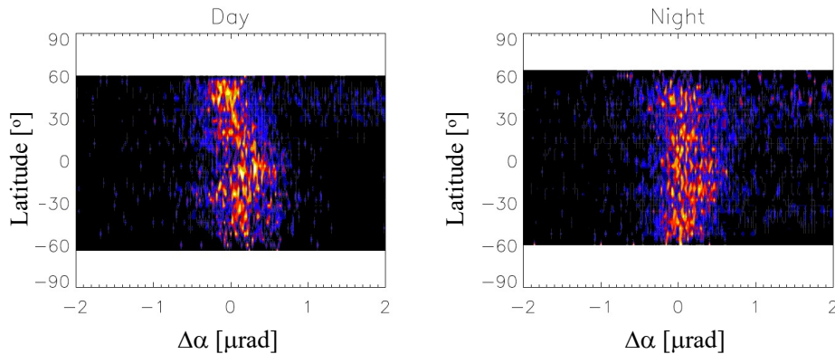
Fig.9 As in Fig.5 for FY3-E from Jan 2023.
