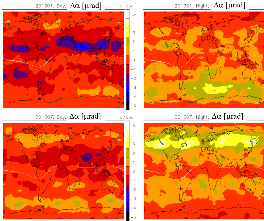
Fig.13. Geographical maps of the \Delta\alpha derived from COSMIC-1 -d\phi_{exL1}/dh_t measurements for January and July 2013; the white lines display positions of the geomagnetic equator. All color numbers have a scale factor indicated at the top of each colorbar.
