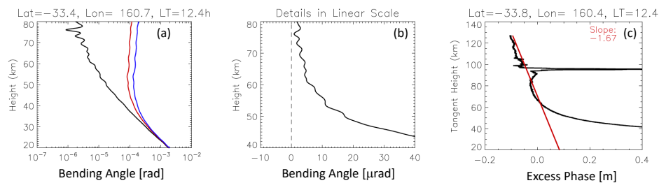
Fig.4. As in Fig.1 but for a case with a sharp spike in the \phi_{ex} profile near 95 km and a significant derivative d\phi_{ex}/dh_t .
