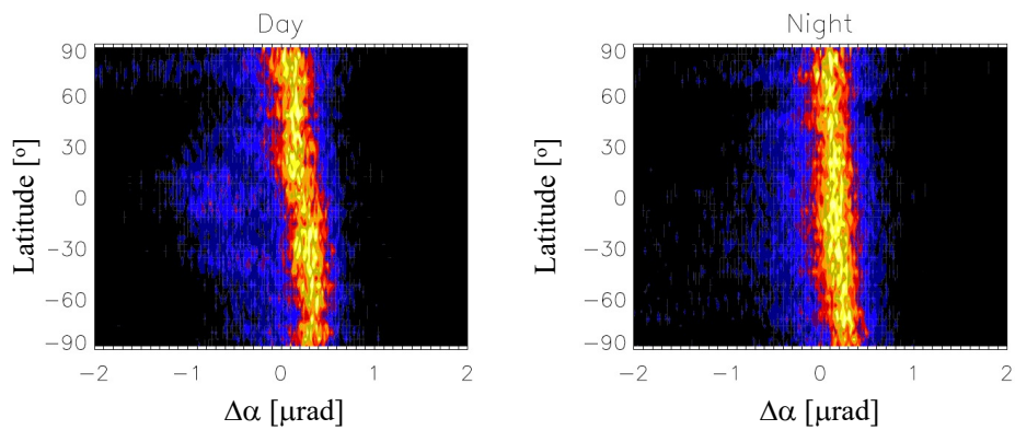
280 Fig.7. As in Fig.5 for Spire from Jan 2022.
