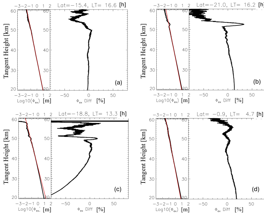
Fig.17. Examples of the departure of excess phase ( \phi_{ex} ) measurements from an exponential fit (red line) at 40-45 km heights.
