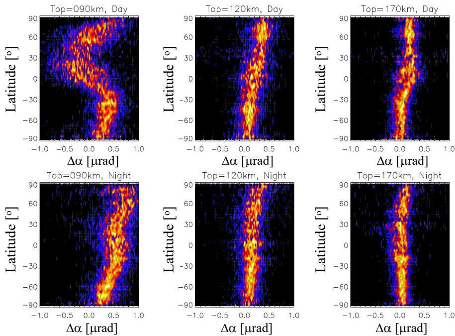
Fig.16. Probability distribution function (PDF) of the RIE derived from the -d\phi_{ex}/dh_t algorithm to compare impacts of the RO top height truncation. The experimental data from the MetOp-A special scan during D161-D254 in 2020 were used in the analysis and the RIE statistics from day (top panels) and night (bottom panels) are reported separately. The RIE results from three RO cutoff top heights, 90, 120, and 170 km, are selected for comparisons.
