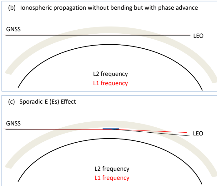
Fig.A1. Illustration of radio wave propagation through an idealized ionosphere (a) with and (b) without bending. A sharp vertical gradient in ionospheric electron density can induce a significant bending, whereas the bending is small and negligible if the gradient is weak. Case (a) illustrates the bending from a sharp refractivity gradient between the vacuum and an ionospheric layer. Case (b) assumes a smooth/gradual transition between the vacuum and the ionosphere such that bending is negligible. In both cases the phase advance is significant and non-negligible (see text for more description).
