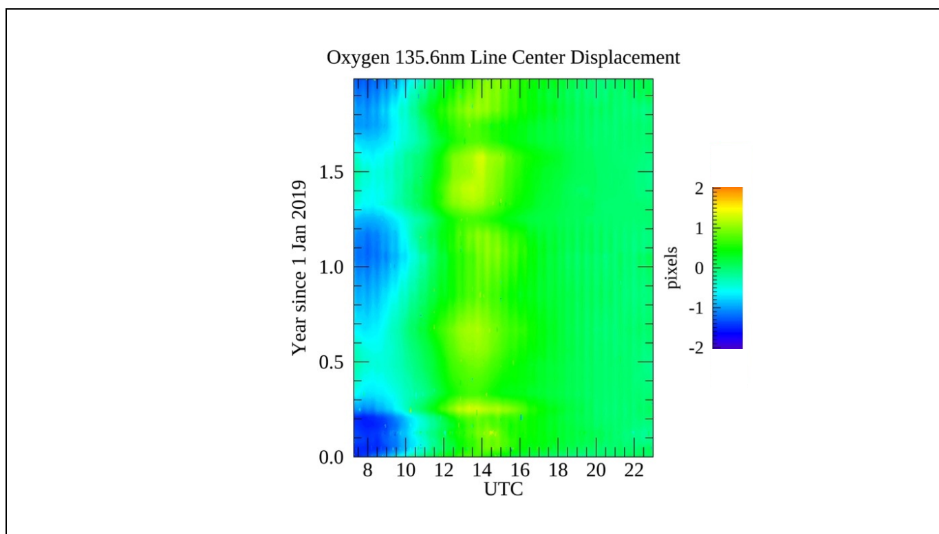
Figure 1: Changes in the peak pixel for the OI 135.6 nm line observed by GOLD throughout each day during 2019 and 2020. The wavelength scales included in the LIC data for each scan decrease the deviations to \sim 0.2 \text{ \AA} ( \sim 1/2 pixel).
