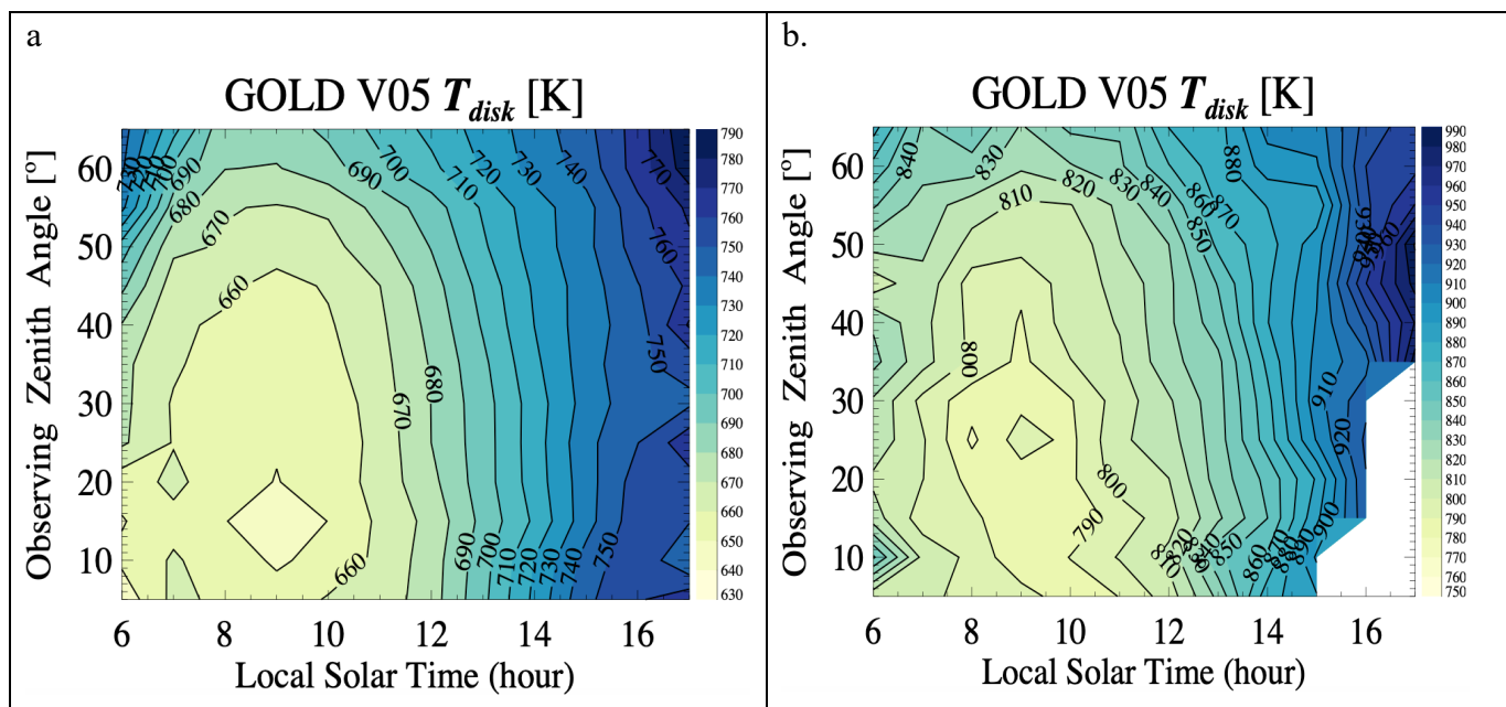
Figure 4: Disk temperatures retrieved from the observations as function of observing zenith angle versus Local solar time (LST) on (a) 2-8 November 2018 (same data as Fig. 3a and including some geomagnetically active days) near solar minimum and on (b) 4-5 November 2022, two geomagnetically quiet days near solar maximum.
