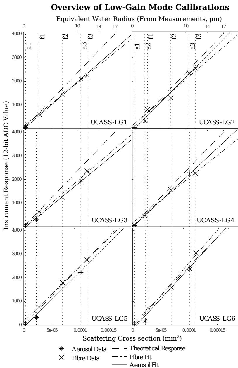
Figure 6. Overview of the calibrations for the low-gain UCASS units. The instrument response is on the y-axis and scattering cross section is on the bottom x-axis. The top x-axis on all the plots is a log axis and shows to the approximate radius of a water droplet with a scattering cross section corresponding to the lower x-axis. The vertical dotted lines highlight the calibration particles used, and the label corresponds to the table entry in Tables 1 and 2
