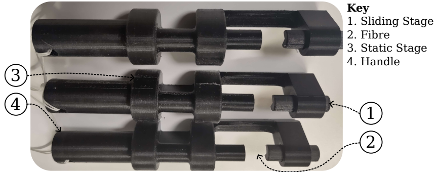
Figure 3. A picture of the custom designed fibre mounts which were used to insert the fibres into the UCASS laser beam for the duration of the calibration. The two stages of the fibre holder and the place for the fibre are labeled.
