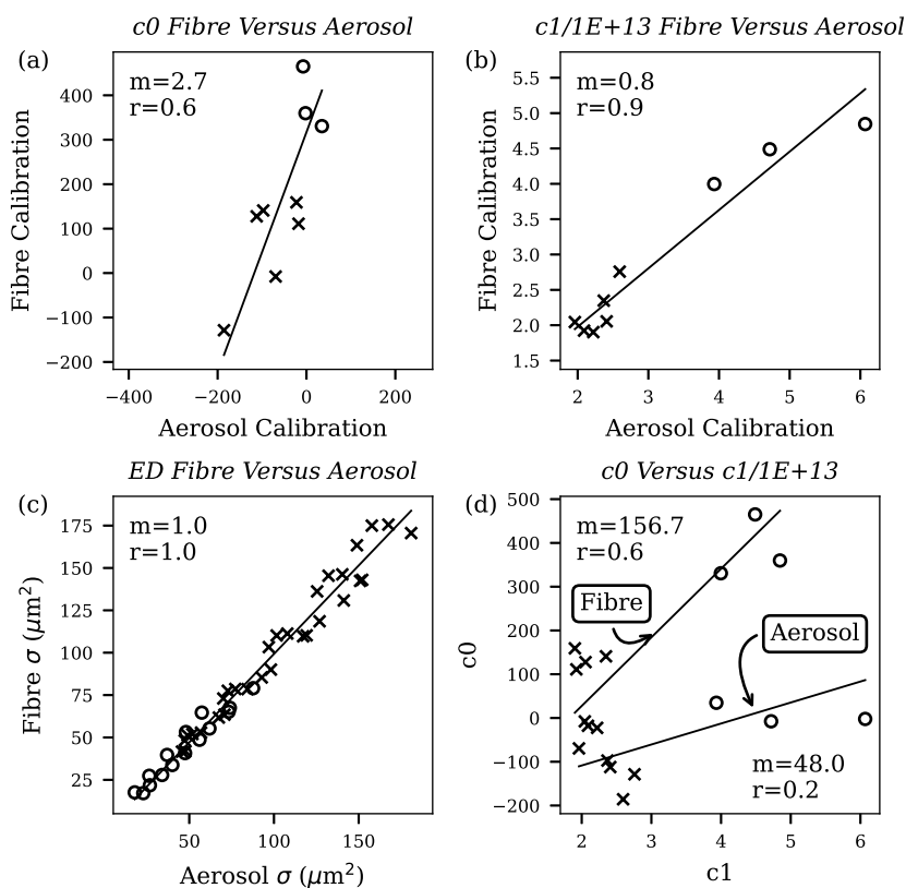
Figure 8. Correlation plots for all of the calibrations. (a) shows the 0 th coefficient for measured for the fibre and aerosol calibrations; (b) shows the same but with the 1 st coefficient; (c) shows the difference in effective diameter computed from a simulated Gaussian distribution with unity standard deviation, with varying initial effective diameter; and (d) shows the 0 th coefficient correlated with the 1 st coefficient for both calibrations.
