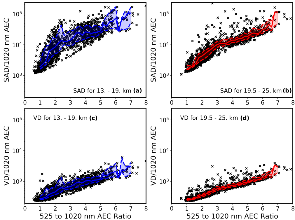
Figure 4. (a) and (b) show SAD/1020 nm aerosol extinction coefficient ( AEC ) to 525/1020 nm aerosol extinction ratio for the low and high altitude group respectively. The dashed lines show the 20 th and 80 th percentile values in bins of 0.2 ratio. The solid line shows the median values. (c) and (d) are the same as (a) and (b) but show VD/1020 nm extinction coefficient to 525/1020 nm extinction ratio.
