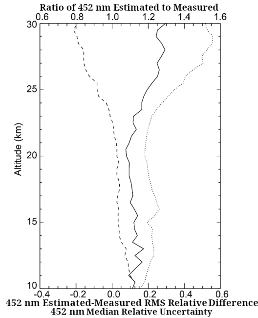
Figure 2. For the Northern Hemisphere ( >20^\circ N) in April 1999 at 452 nm: 1) ratio of estimated to measured aerosol extinction coefficient (dashed, top scale), 2) relative RMS mean difference between estimated and measured aerosol extinction coefficient (solid, bottom scale). 3) median relative aerosol extinction coefficient measurement uncertainty absolute value (dotted, bottom scale).
