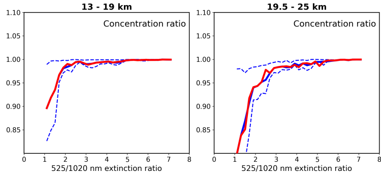
Figure 7. The five parameters defining a bimodal size distribution are shown for 13-19 (left) and 19.5-25 (right) km same as a function of the 525/1020 nm extinction ratio. The median (bold blue) Figure 5 and 20 th and 80 th percentile (dashed blue) values are shown Figure 6 but for each extinction the concentration ratio bin. Results of the swarm optimization fit are shown in red.
