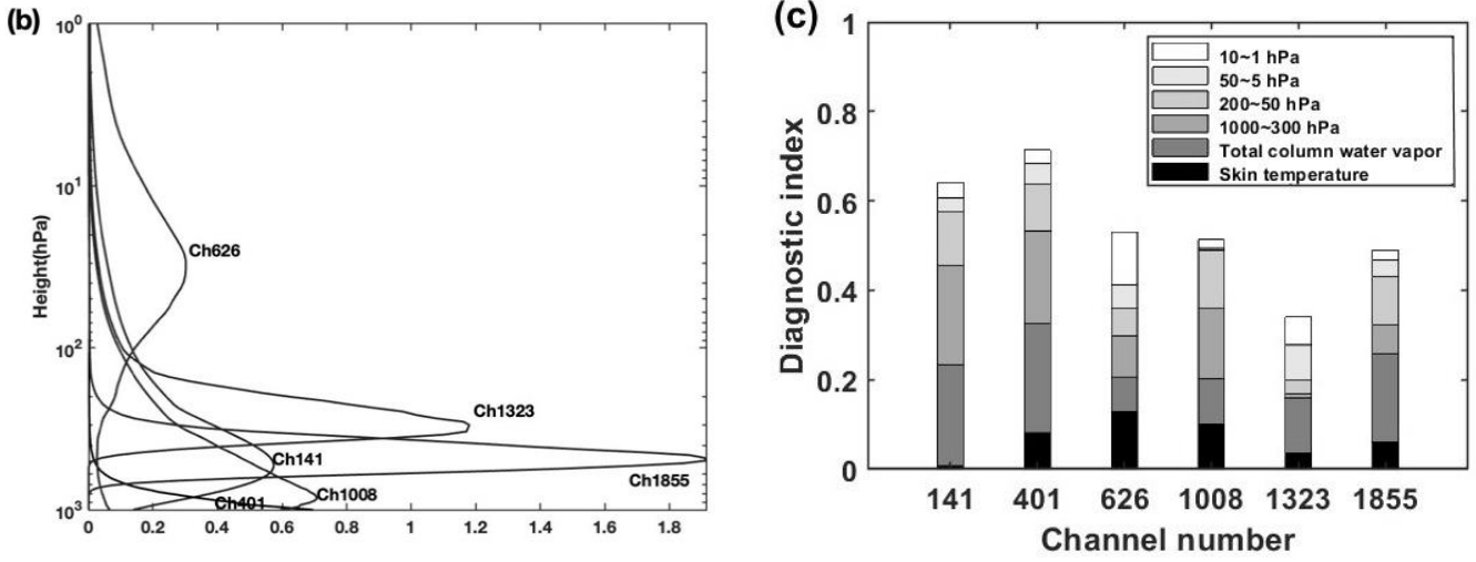
Fig. 1. (a) Simulated HIRAS-II brightness temperature spectrum (black curve) by the RTTOV using the US76 standard atmospheric profile, the selected 6 typical channels (red dots) and the assimilated 485 channels (black dots). (b) weighting function of the selected channels. (c) relevance diagnostics of bias-correction.
