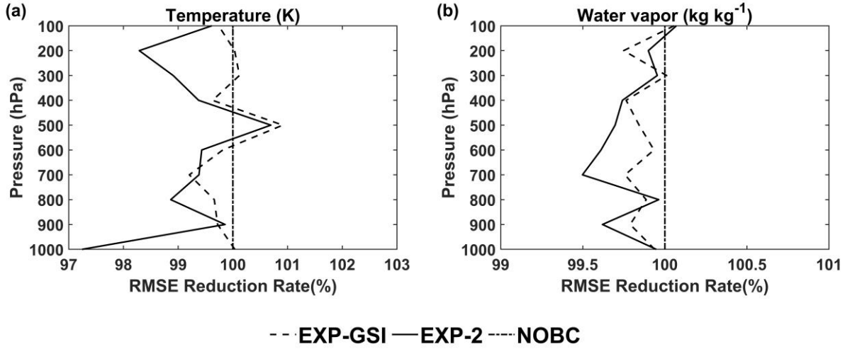
Fig. 8 Averaged vertical RMSE profiles of (a) temperature and (b) specific humidity compared with ERA5. The vertical RMSE profiles are normalized by the RMSE from the NOBC experiment.
