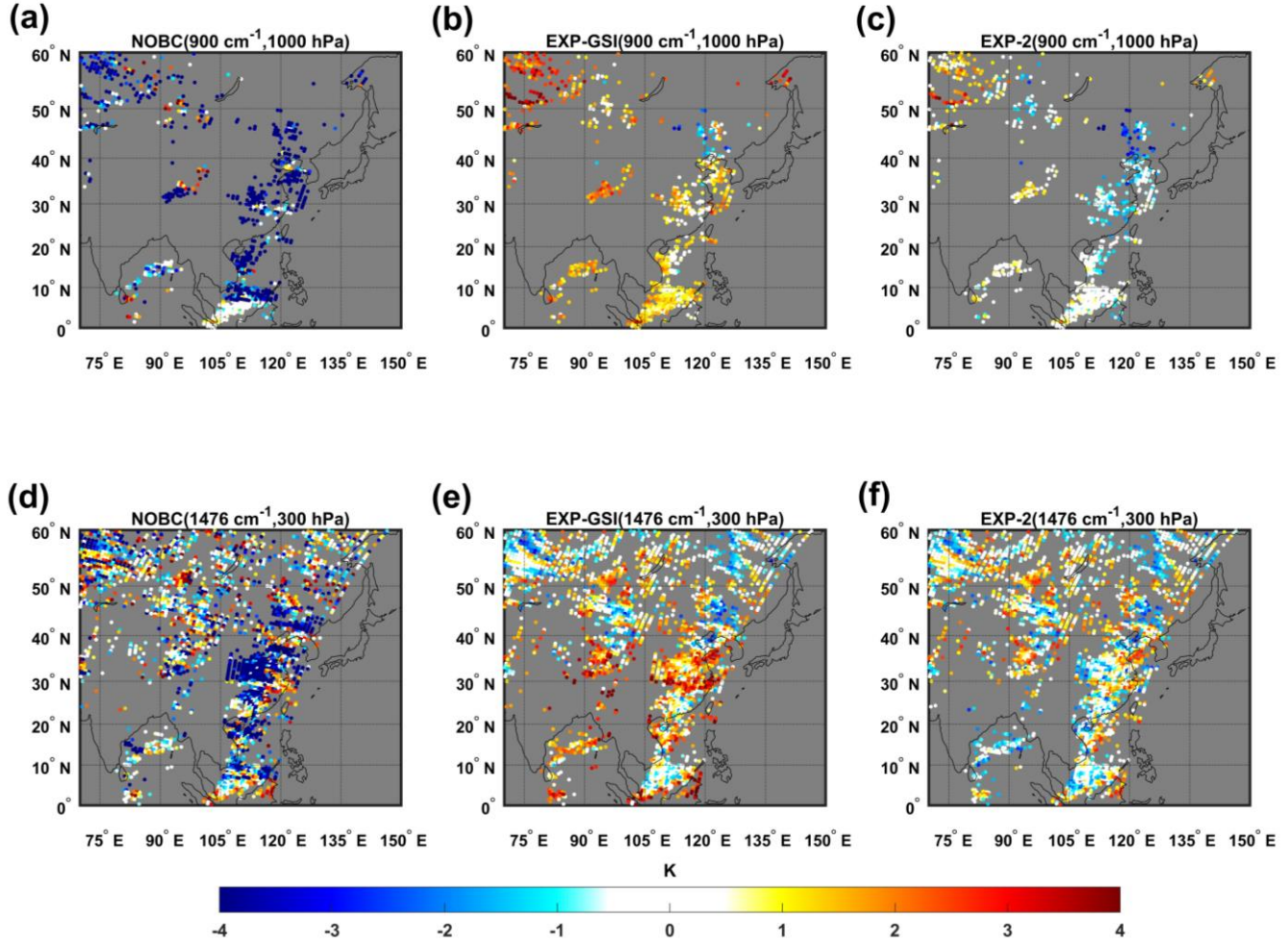
393 Fig. 7 Spatial distributions (colored dots) of the HIRAS-II O-B biases without BC (left), with the EXP-GSI BC (middle) and 394 with the EXP-2 BC (right) for (a)~(c) the 900 \text{cm}^{-1} channel (1000 hPa) and (d)~(f) 1476 \text{cm}^{-1} channel (300 hPa) at 0000 UTC 7 395 August 2023.
