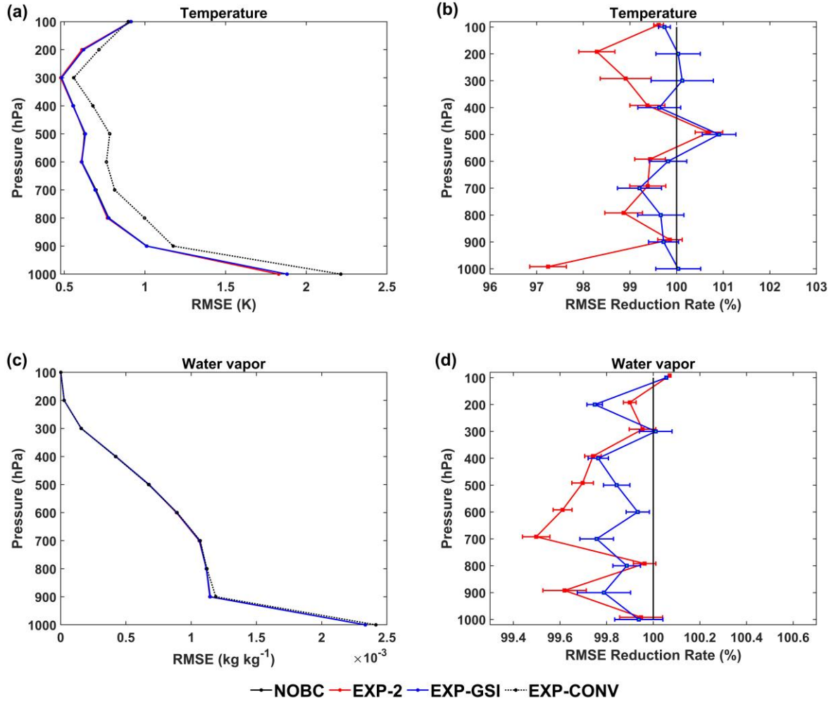
414 415 Fig. 8 Averaged vertical RMSE profiles of (a) temperature and (c) water vapor compared with ERA5. The vertical RMSE profiles 416 of (b) temperature and (d) water vapor are normalized by the RMSE from the NOBC experiment. Error bars give statistical 417 significance intervals for differences from the NOBC at the 95% level.
