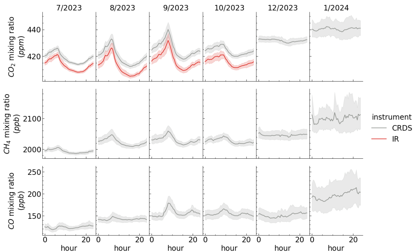
Figure 4. Monthly dry mixing ratios diel pattern for all measured gases (CO 2 , CH 4 and CO) for IR (LI-7200) and CRDS (PICARRO G2401). Solid line indicates median and region shows 95% confidence interval.
