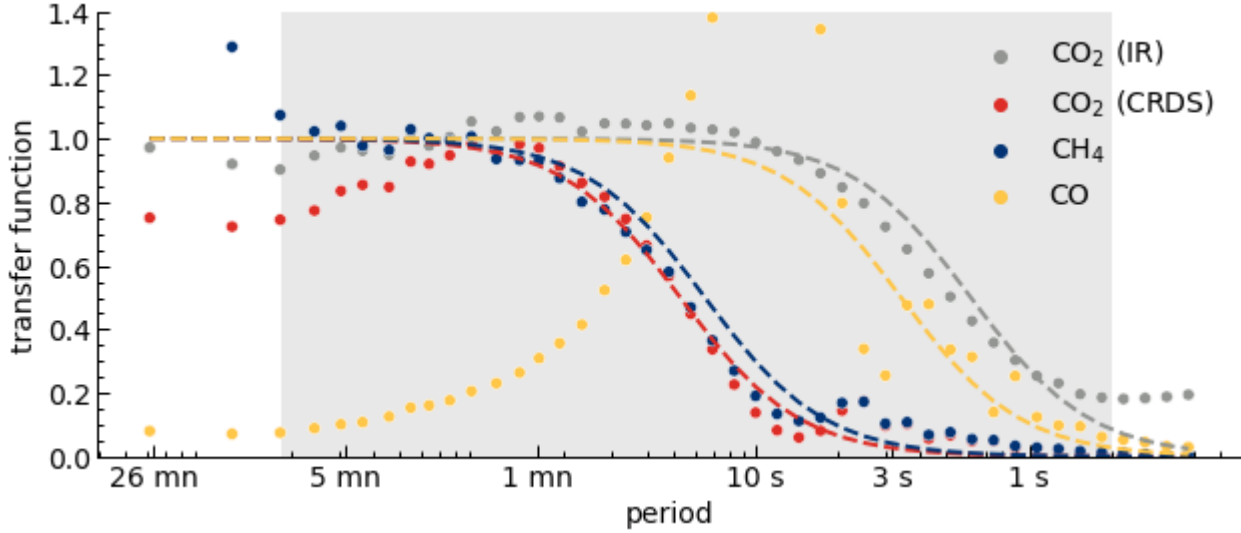
255 Figure 3. Transfer functions H (dotted lines) for each compound and analyser. The transfer function was fitted to the ratio of each compound's spectra to the sonic temperature spectra. All spectra are ensemble averaged taken from EddyPro outputs, filtered for significant fluxes. Dots show the mean spectra per frequency band. The grey shaded area show the frequency range (2 - 0.0018 Hz) over which transfer functions were fitted. See figure S1 for more detailed power spectra.
