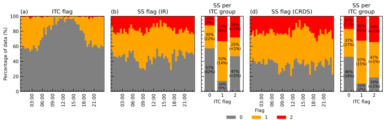
Figure 8. Quality control flags for turbulence (ITC) and CO 2 stationarity (SS). Flags follow 0-1-2 system for high, medium and low-quality. Percentage of (a) turbulence flagged data by hour of the day. Stationarity flagged CO 2 data by hour of the day for the (b) the Licor instrument (IR) and (d) the PICARRO instrument (CRDS). Stationarity flag per ITC group are also given for the IR (b) and CRDS instrument (c). Percentages are summed to 100% in each group and over all data (in parentheses).
