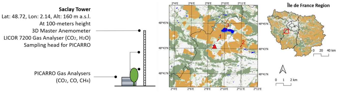
Figure 1. Site diagram showing tower and acquisition house and tree for scale. On the right panel, site map and localisation in the region. Colours indicate land use: cropland (orange); grassland (light green); forest (dark green); water (light blue); white (urban). For reference (1) heating plant, (2) manure/composting plant, (3) lake.
