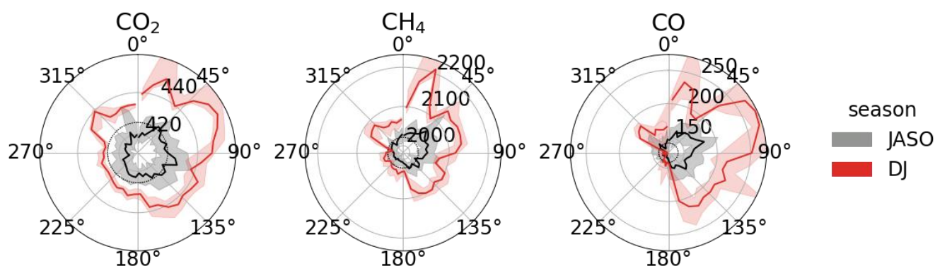
Figure 5. Median dry mixing ratios by wind direction, band shows interquartile 25 th and 75 th percentiles. Warmer months (July to October) in grey and colder months (December and January) in red. Extreme values in the left and right 0.1% tails were removed. See Figure S2 for monthly observations. CO 2 is in ppm while CH 4 and CO are in ppb. All data, including non-stationary and underdeveloped turbulence.
