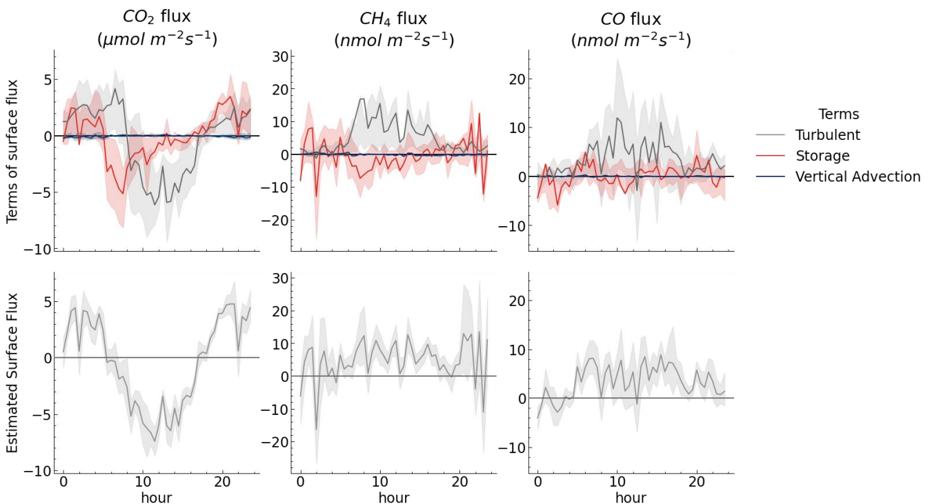
Figure 15. Diel mean for CO 2 , CH 4 and CO turbulent, storage and vertical advection fluxes in the top panel and their sum, i.e. estimated surface flux on bottom panel. Data for July 2023. Values for the CRDS (PICARRO G2401). Band shows interquartile (25 th - 75 th percentiles). See Figure S9 for all months.
