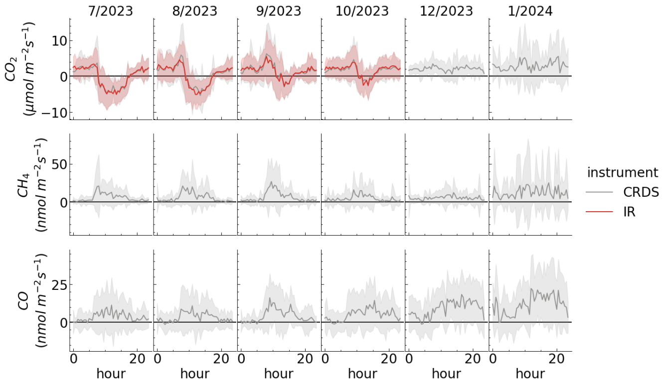
Figure 11. Monthly mean turbulent fluxes diel pattern of CO 2 , CH 4 and CO for IR (LI-7200, only CO 2 ) and CRDS (PICARRO G2401) gas analysers. Fluxes shown after spectral correction. Data points falling within the extreme 1% tail of the distribution were removed. Shaded area refers to standard deviation.
