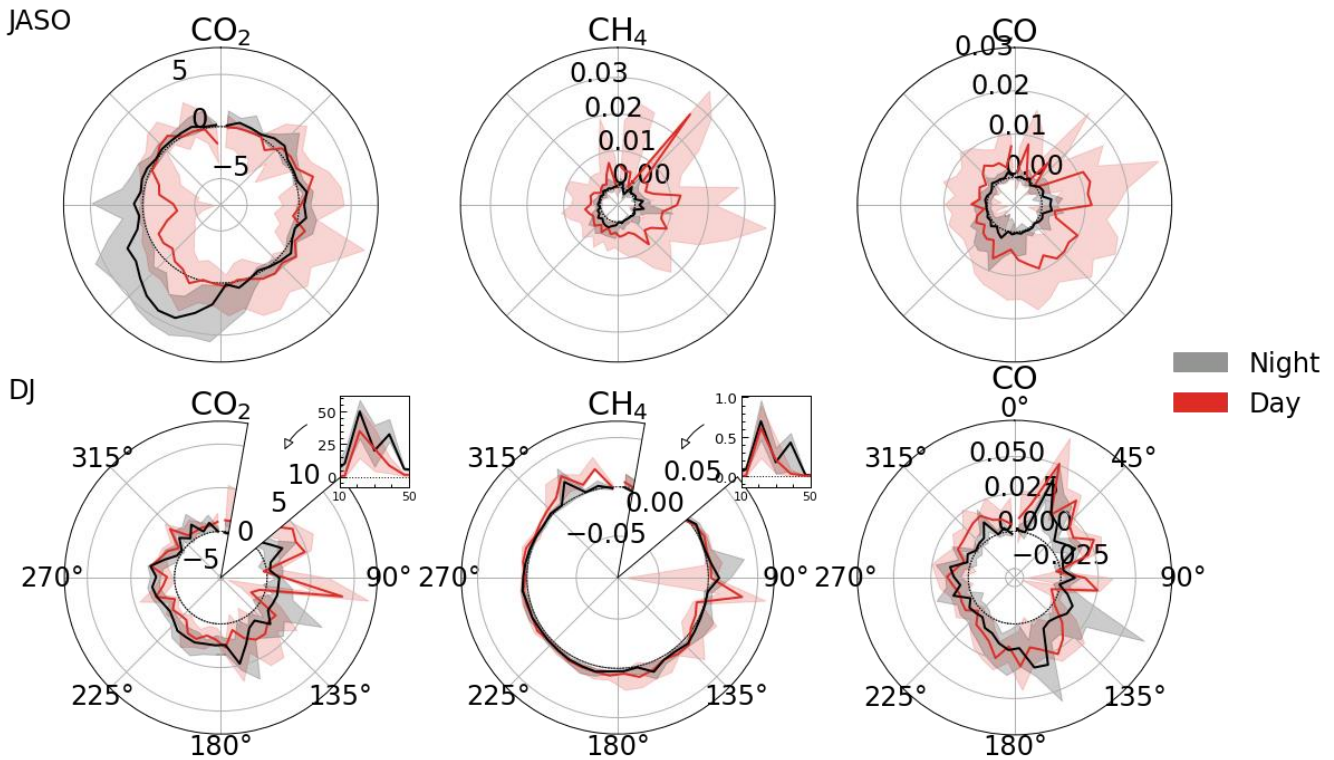
Figure 12. CO 2 , CH 4 and CO turbulent fluxes by wind direction. Warmer months (JASO) in the top panel, and colder months (DJ) in the bottom. The values are the median with the interquartile range in the shaded area, 0.1% extreme values were removed. Wind directions bins with less than 10 observations were added to the next bin clockwise. CO 2 fluxes are in \mu\text{mol m}^{-2} \text{s}^{-1} and fluxes of CH 4 and CO are in \text{nmol m}^{-2} \text{s}^{-1} . Note that 10-50° for CO 2 and CH 4 in December and January were plotted separately for visual purposes. See Figure S4 for monthly values. Only stationary periods and with well-developed turbulence are considered.
