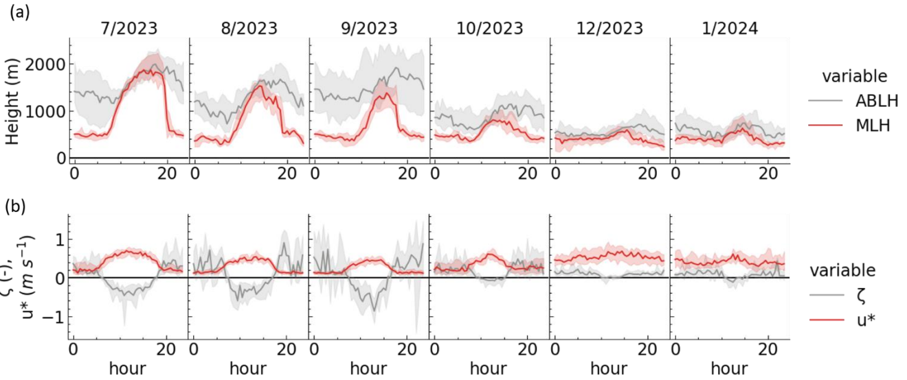
Figure 7. Boundary layer conditions. (a) Heights of the atmospheric boundary layer (ABLH) and the mixing layer (MLH) measured by SIRTAs in Palaiseau, 4.8 km away from the tower. Data available online (Kotthaus et al., 2023). (b) Stability parameter ( \zeta = (z - d) / L ) and friction velocity ( u^* ) measured at the FR-Sac tower. Absolute values of \zeta bigger than 2 were ignored.
