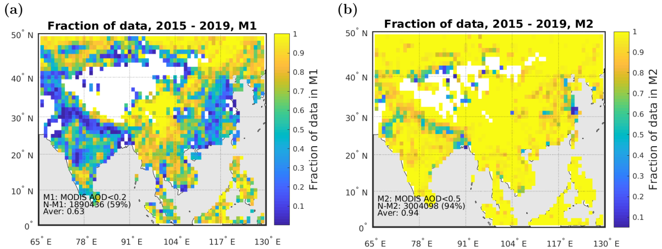
Figure 9. Difference in using MODIS AOD threshold 0.2 or 0.5 in Asia. Panels a) and b) show the fraction of data in M1 or M2, respectively, for each 1^\circ \times 1^\circ grid cell.
