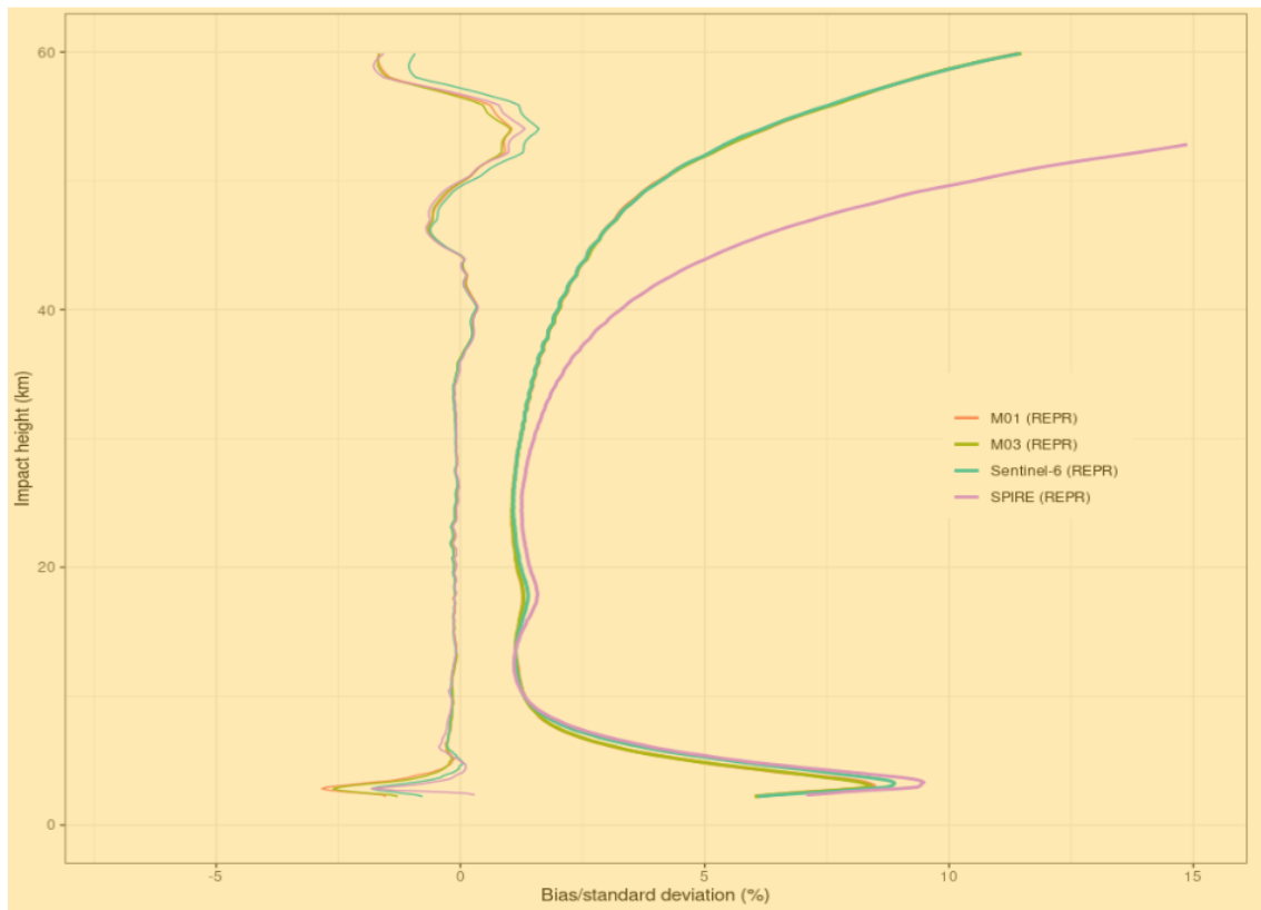
Figure 17. Global robust statistics of reprocessed GRAS (M01/B and M03/C), Spire and Sentinel-6A bending angles compared against ECMWF short range forecasts during the analyzed period. The vertical profiles of biases (or systematic deviations) with thin lines and respective standard deviations (or random deviations) are shown for the different missions.
