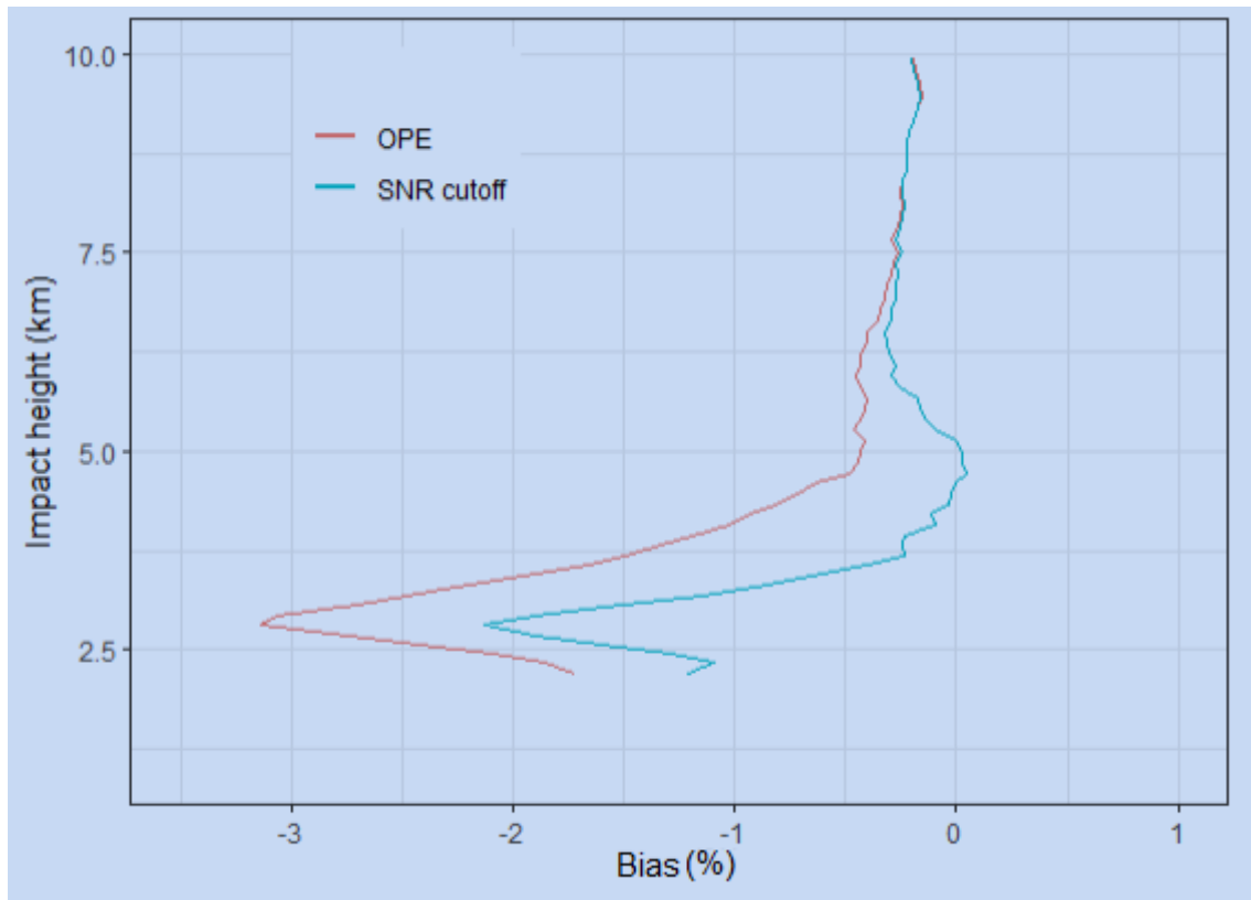
Figure 8. Global robust statistics of S6 bending angles compared against ECMWF short range forecasts during the analyzed period. Only vertical profiles of biases (or systematic deviations) in troposphere are shown for operational and reprocessed data employing the SNR-based cutoff algorithm.
