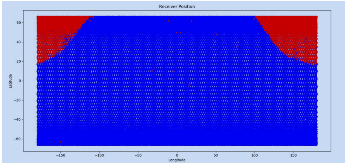
Figure 15. Receiver position for Sentinel-6A occultations affected by the interference signals in the L2 frequency, in the period between August 2021 and May 2022.
