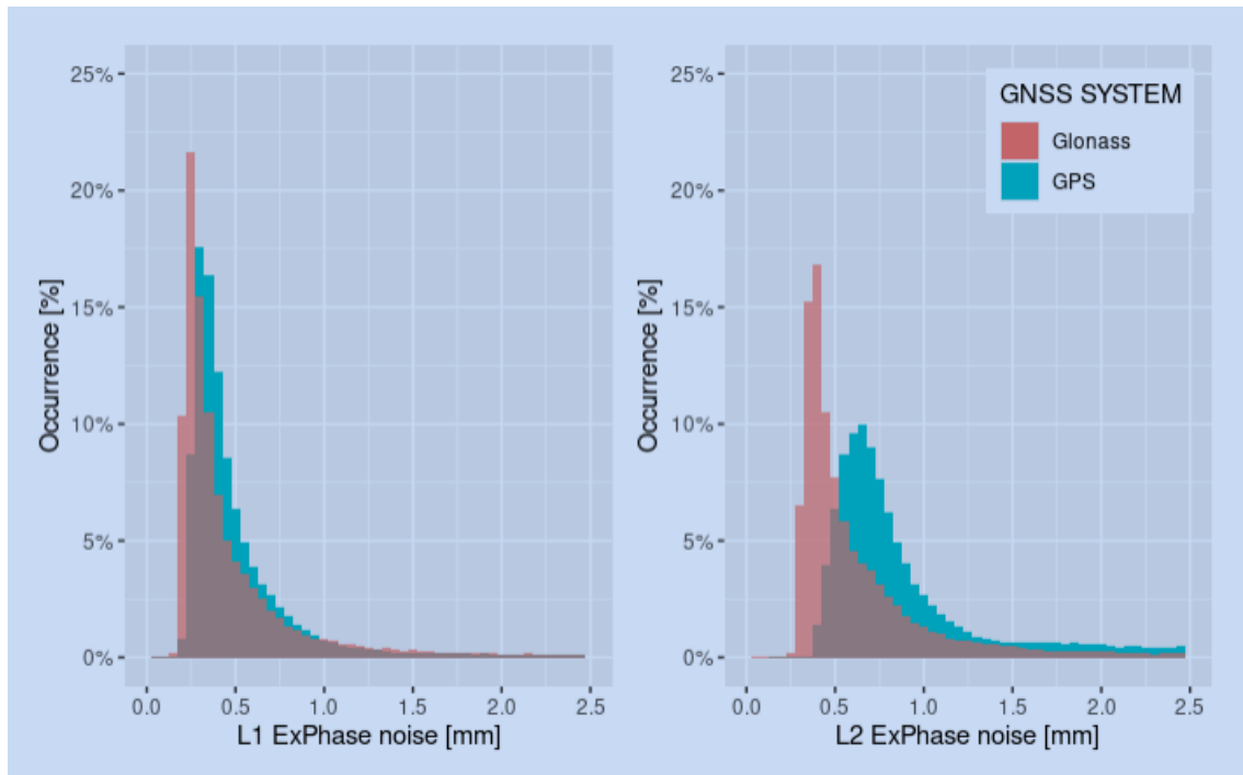
Figure 7. Histograms of Excess Phase noise measured between 60 and 80 km SLTA split per constellation, for L1 (left) and L2 (right) frequencies.
