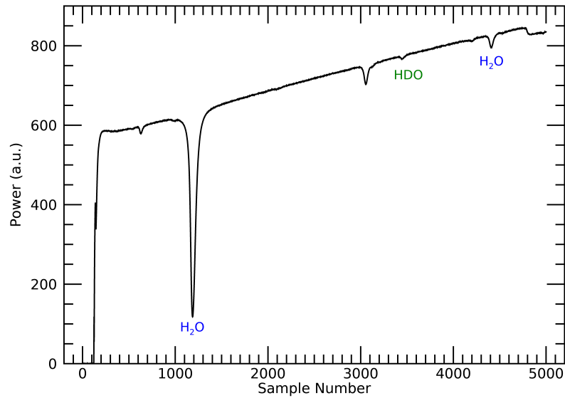
Figure 1. Spectrum showing the three major absorption features used for ChiWIS water isotope measurements. Samples are taken at 2.5 microsecond intervals. Shown here is a 2-s spectrum 2-second average of spectra taken during the StratoClim campaign (Flight 6, August 6, 2017) in air with about \sim 50 ppmv water vapor; the HDO line is about 0.8% deep relative to an assumed linear baseline . The \text{H}_2\text{O} feature at 3777.949\text{ cm}^{-1} centered at sample 1200 is used for dry air in the UTLS ( mixing ratios can reach approximately 4 ppmv ), but becomes optically saturated and difficult to fit at high mixing ratios; in these conditions we use the smaller water feature at 3777.44\text{ cm}^{-1} centered at sample 4500. The feature at sample 4800 is a mode hop, an instrumental artifact due to the laser diode rapidly switching from one longitudinal mode to another . See Table 2 for properties of each absorption features.
