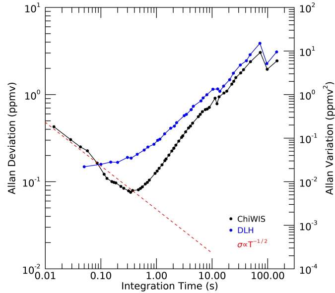
Figure 10. The flush-instrument response time of the optical cavity is estimated via an Allan deviation plot constructed using flight data from a flight leg with very high natural-variabilityatmospheric variability . The open-path Diode Laser Hygrometer (DLH) (Diskin et al., 2002) instrument (blue) measures natural-atmospheric variability down to the shortest integration time reported, 0.05 seconds. The ChiWIS instrument (black) involves a well-mixed optical cell; at short timescales signal averaging produces gains in sensitivity. The turnaround at 0.5 seconds suggests this is the characteristic flush-response time of the cell-instrument and natural-atmospheric variability dominates at larger timescales.
