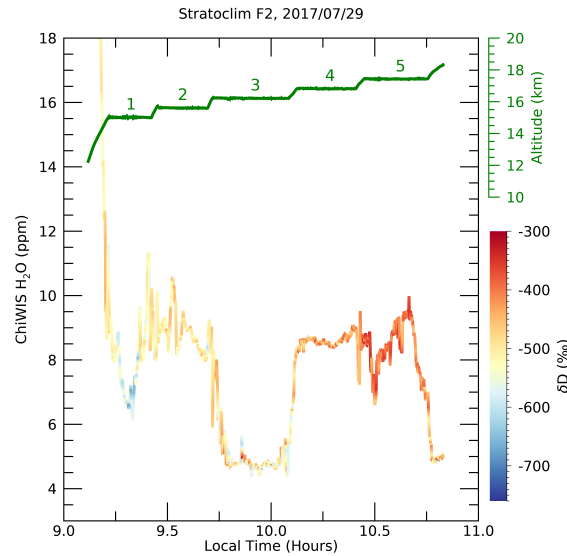
Figure 15. Illustration of natural -atmospheric isotopic variations detectable in flight data. Figure shows water isotope measurements from Flight 2 of the StratoClim campaign; on this flight the aircraft flew five level flight legs between 15 and 17.5 km (green). The second, fourth, and fifth flight legs all feature \text{H}_2\text{O} mixing ratios of \sim 8.5 ppmv, but have significantly different isotopic ratios, reflecting their distinct origins: \delta\text{D} means and standard deviations of -503 \pm 28\text{‰} , -436 \pm 30\text{‰} , and -398 \pm 32\text{‰} , respectively. In contrast, legs two and three show significantly different water vapor values but nearly identical \delta\text{D} of -503 and -508\text{‰} , respectively.
