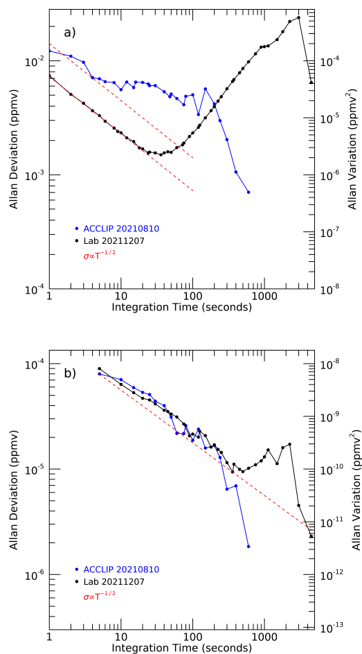
Figure 8. Allan deviation plots for measured H 2 O (a) and HDO (b) mixing ratios in laboratory (black) and flight (blue) conditions. Lab deviations are constructed from 2.75 hours of data taken on on ultra-dry air (mean mixing ratios of 2.51 ppmv H 2 O and 760 pptv HDO). Flight deviations are constructed from 1166 seconds (~20 minutes) of data taken during a level flight leg at 18.3 km with relatively constant water vapor (mean mixing ratios of 3.46 ppmv H 2 O and 890 pptv HDO). In the laboratory data, the maximum achievable precision for H 2 O is 1.5 ppbv with 40-s integration; for HDO it is 10 pptv at 500-s integration. In both cases, integration effects up to these thresholds resemble those expected that from the averaging of purely Gaussian noise (red dashed lines, proportional to T^{-1/2} ). Beyond these thresholds the deviations increase, likely due to the presence of a long-period fringe. In the flight data, Allan deviations for HDO are similar to those in the lab, but for H 2 O are about twice as large and relatively constant, likely reflecting real atmospheric variations above the sensitivity threshold of the measurement.
