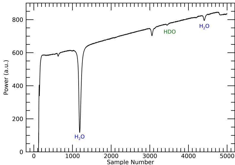
Figure 1. Spectrum showing the three major absorption features used for ChiWIS water isotope measurements. Samples are taken at 2.5 microsecond intervals. Shown here is a 2-second average of spectra taken during the StratoClim campaign (Flight 6, August 6, 2017) in air with about \sim 50 ppmv water vapor; the HDO line is about 0.8% deep relative to an assumed linear baseline. The \text{H}_2\text{O} feature at 3777.949\text{ cm}^{-1} centered at sample 1200 is used for dry air in the UTLS (mixing ratios can reach approximately 4 ppmv), but becomes optically saturated and difficult to fit at high mixing ratios; in these conditions we use the smaller water feature at 3777.44\text{ cm}^{-1} centered at sample 4500. The feature at sample 4800 is a mode hop, an instrumental artifact due to the laser diode rapidly switching from one longitudinal mode to another. See Table 2 for properties of each absorption features.
