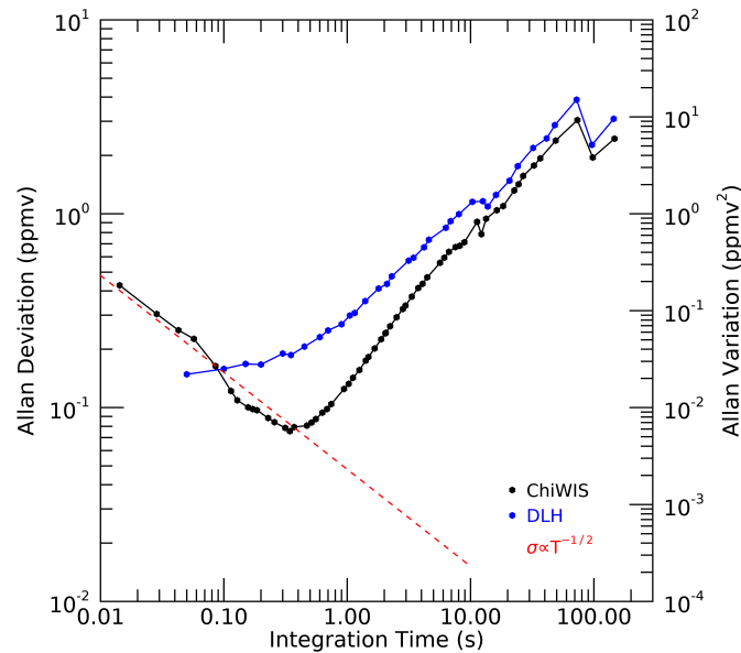
Figure 10. The instrument response time is estimated via an Allan deviation plot constructed using flight data from a flight leg with very high atmospheric variability. The open-path Diode Laser Hygrometer (DLH) (Diskin et al., 2002) instrument (blue) measures atmospheric variability down to the shortest integration time reported, 0.05 seconds. The ChiWIS instrument (black) involves a well-mixed optical cell; at short timescales signal averaging produces gains in sensitivity. The turnaround at 0.5 seconds suggests this is the characteristic response time of the instrument and atmospheric variability dominates at larger timescales.
