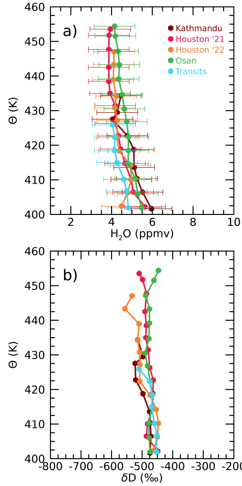
Figure 14. Comparison across campaigns of stratospheric measurements, which should be relatively stable: a ), average stratospheric profiles of water vapor and b ), \delta\text{D} , plotted against potential temperature. Data in both panels are binned into 5 degree potential temperature. Dots represent the mean value of each bin, and horizontal error bars show the standard deviation. All data are taken in summer.
